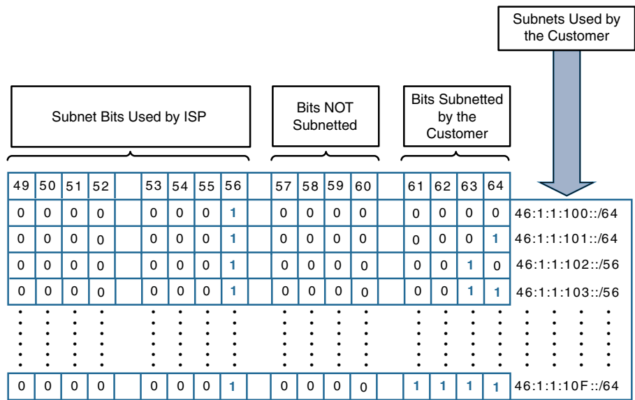
Figure 11-4 Bits Provided to the Customer
