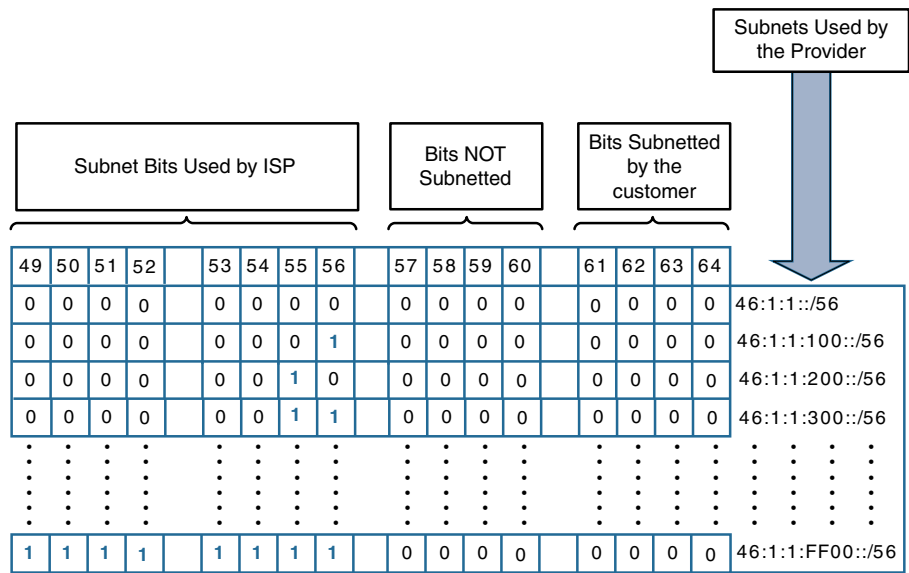
Figure 11-3 Provider Bits Used to Generate /56 Subnets
