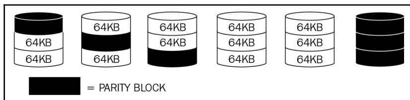
Figure 14: RAID 6
