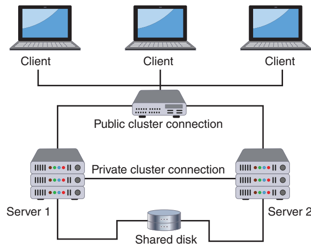
Figure 14-1 Server cluster
