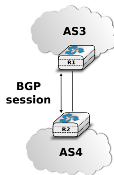
Figure 5.60: A BGP peering session between two directly connected routers
