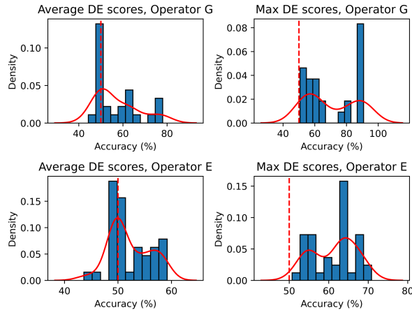
(a) Accuracy distributions for DE locations.
