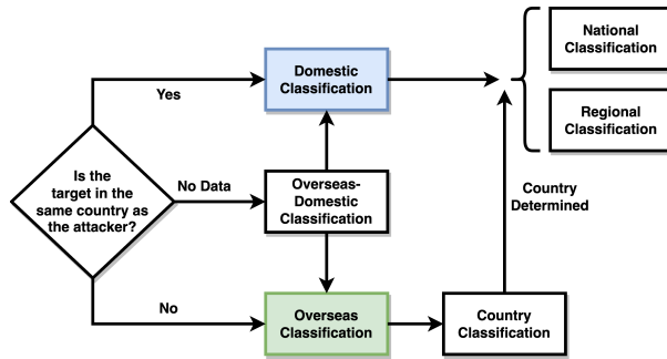
Figure 5: The classification methodology
