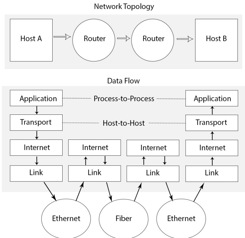
Figure 4.1 – Diagram of a TCP/IP data flow
