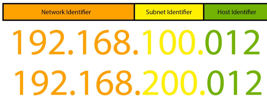
Figure 4.6 – Subnets visualized
