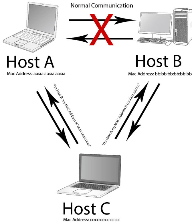
Figure 4.9 – A diagram of an ARP spoof
