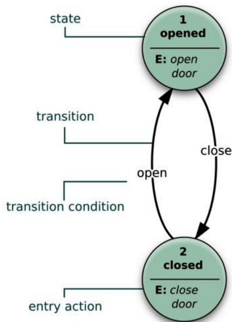
Figure 5.1 – State machine model diagram
