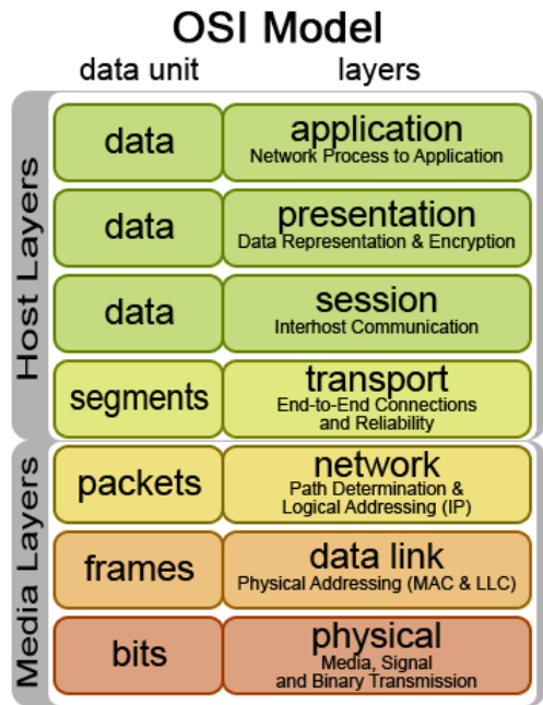
Figure 4.2 – Diagram of the OSI model
