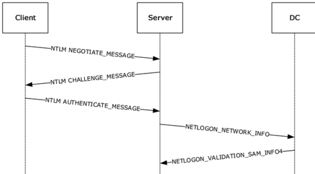
Figure 5.4 – NTLM authentication diagram
