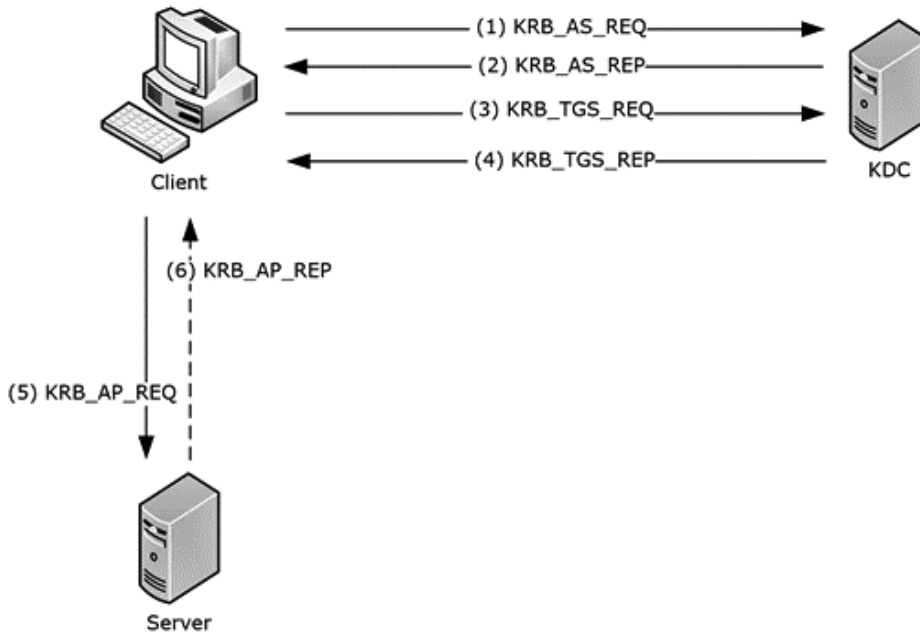
Figure 5.5 – A diagram of Kerberos authentication
