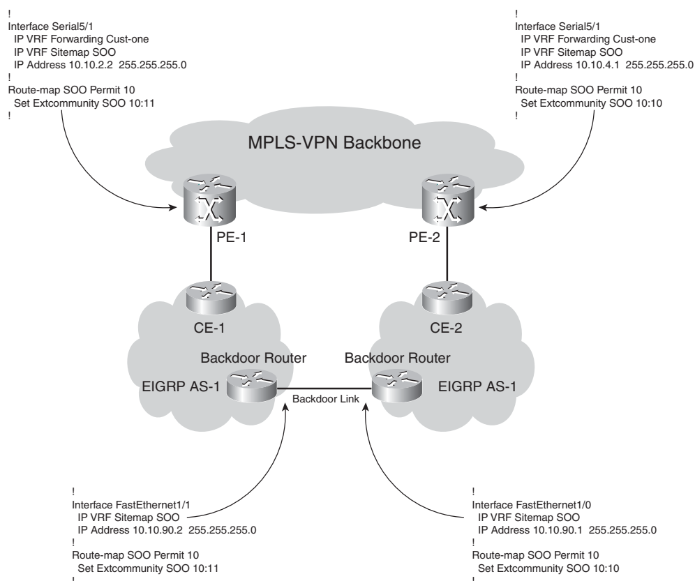
Figure 7-25 Backdoor Link Between EIGRP Sites
