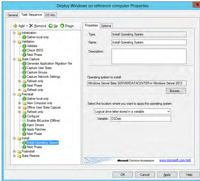
FIGURE 2-7 Customizing a task sequence.
