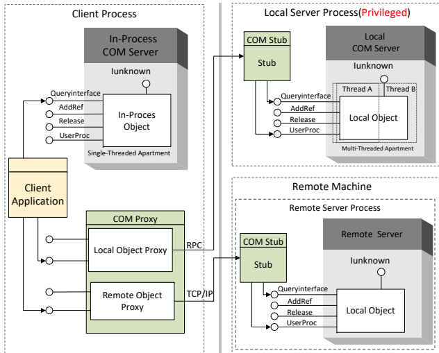
Figure 1: In-process and cross-process COM objects.
