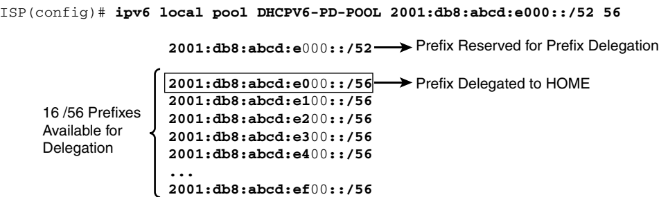
Figure 11-8 ISP's Local Prefix Pool
