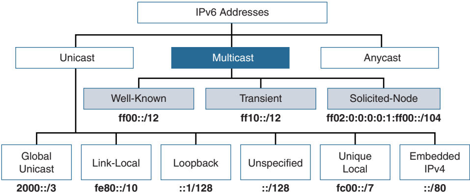
Figure 4-11 Multicast Addresses
