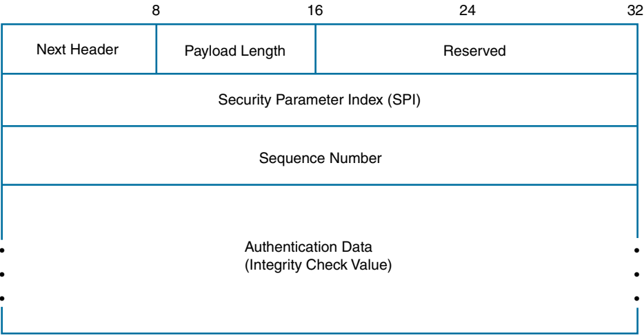
Figure 3-28 AH Extension Header
