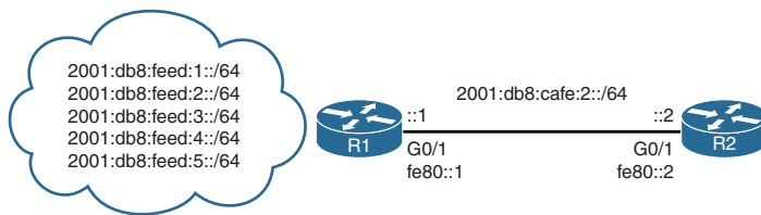
Figure 14-7 R1 Networks
