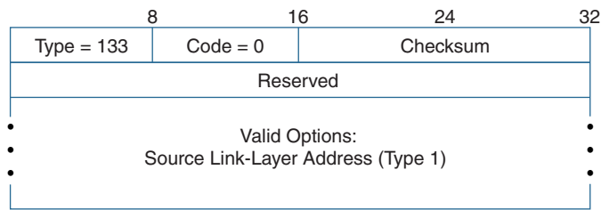
Figure 13-2 ICMPv6 ND Router Solicitation Message
