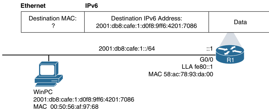
Figure 13-5 Known IPv6 Address but Unknown Ethernet MAC Address
