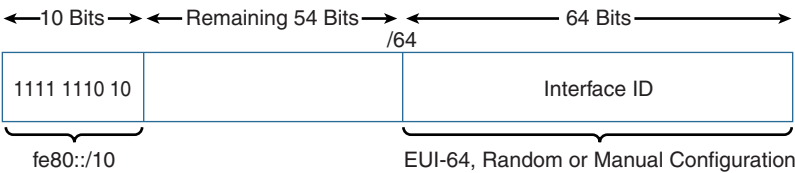
Figure 6-2 Link-Local Unicast Address
