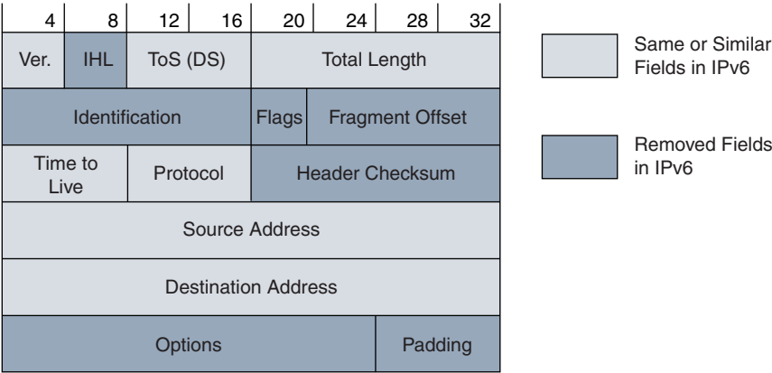
Figure 3-1 IPv4 Header
