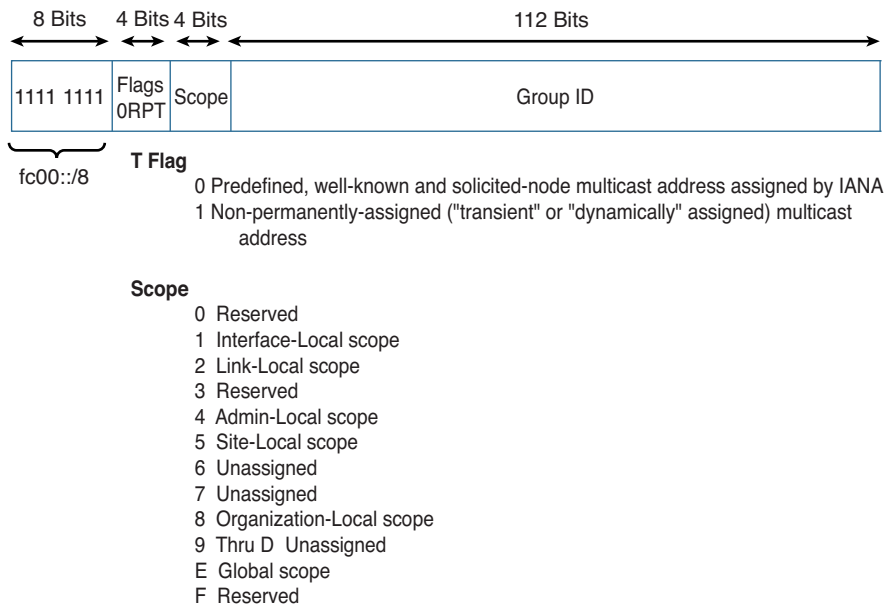
Figure 4-12 IPv6 Multicast Address
