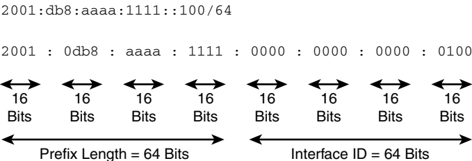
Figure 4-2 IPv6 Prefix and Prefix Length
