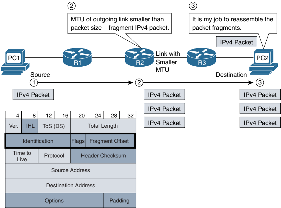
Figure 3-9 IPv4 Fragmentation Fields
