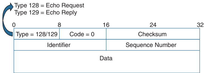
Figure 12-9 ICMPv6 Echo Request and Echo Reply Messages
