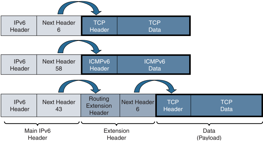
Figure 3-12 IPv6 Next Header Examples
