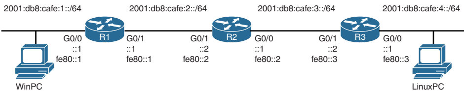
Figure 9-8 Topology for Autoconfigured Address States and Lifetimes Example
