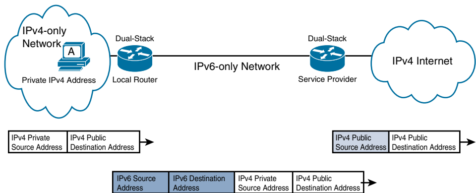
Figure 17-15 Dual-Stack Lite
