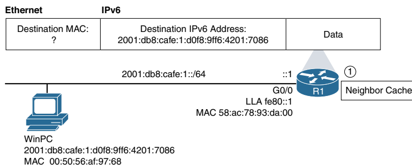
Figure 13-6 R1 Checks Its Neighbor Cache
