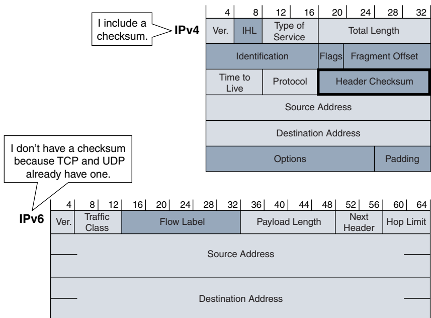
Figure 3-14 IPv4 Checksum Field
