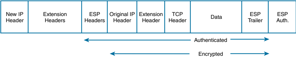
Figure 3-27 ESP—Transport and Tunnel Modes
