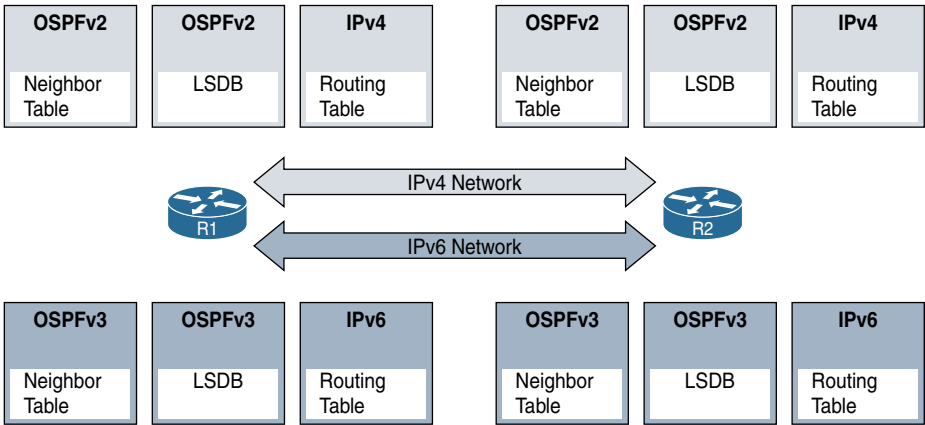
Figure 16-1 Separate Neighbor Tables and LSDBs for OSPFv2 and OSPFv3
