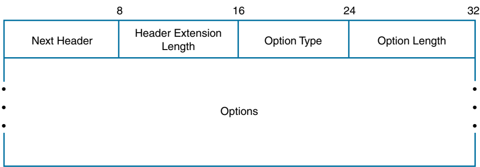
Figure 3-30 Destination Options Extension Header
