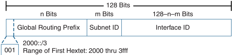
Figure 5-2 Structure of a Global Unicast Address
