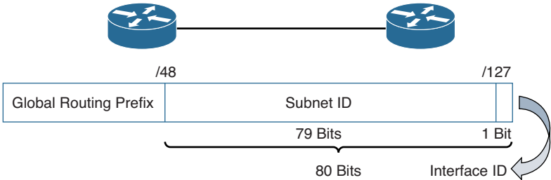
Figure 5-17 /127 Prefix
