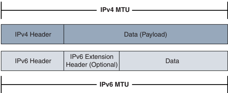
Figure 3-8 IPv4 and IPv6 MTUs
