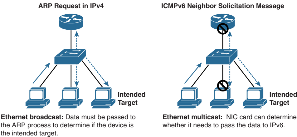
Figure 13-13 ARP Request Versus ICMPv6 Neighbor Solicitation Message
