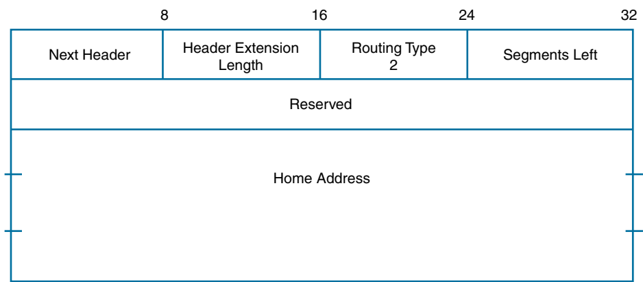
Figure 3-23 Type 2 Routing Header
