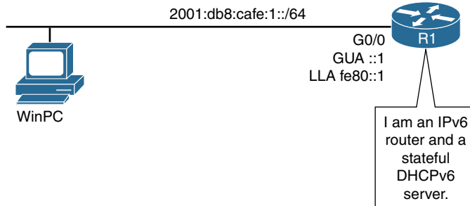
Figure 11-2 Topology for Stateful DHCPv6 Configuration
