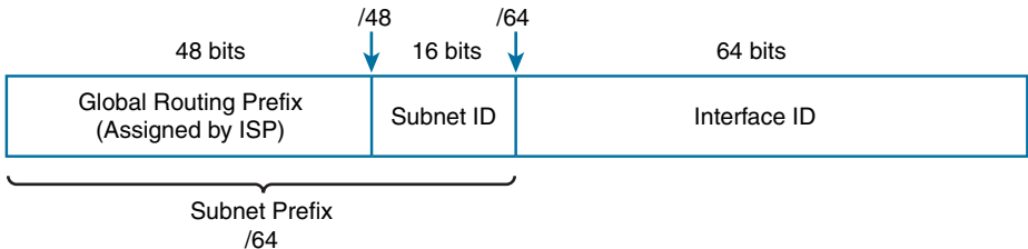
Figure 5-11 Subnet Prefix
