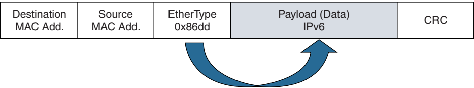
Figure 3-17 IPv6 Packet Encapsulated in an Ethernet II Frame
