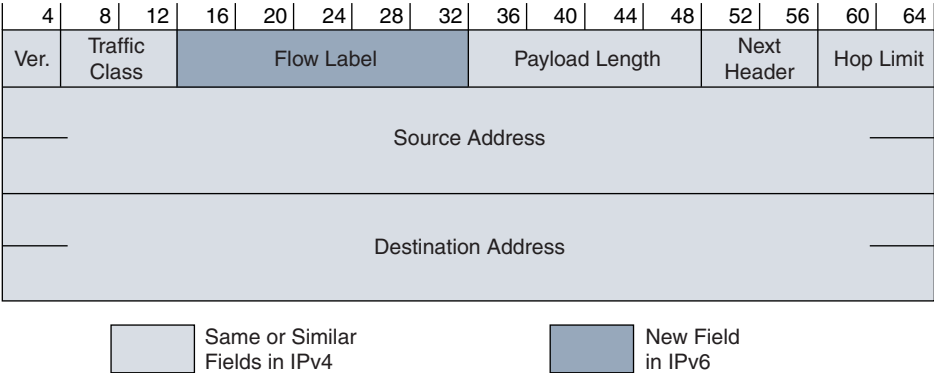
Figure 3-2 IPv6 Header
