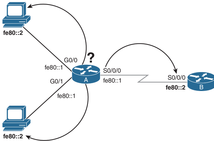
Figure 6-10 Same Link-Local Address on Different Networks
