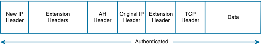
Figure 3-29 AH—Transport and Tunnel Modes
