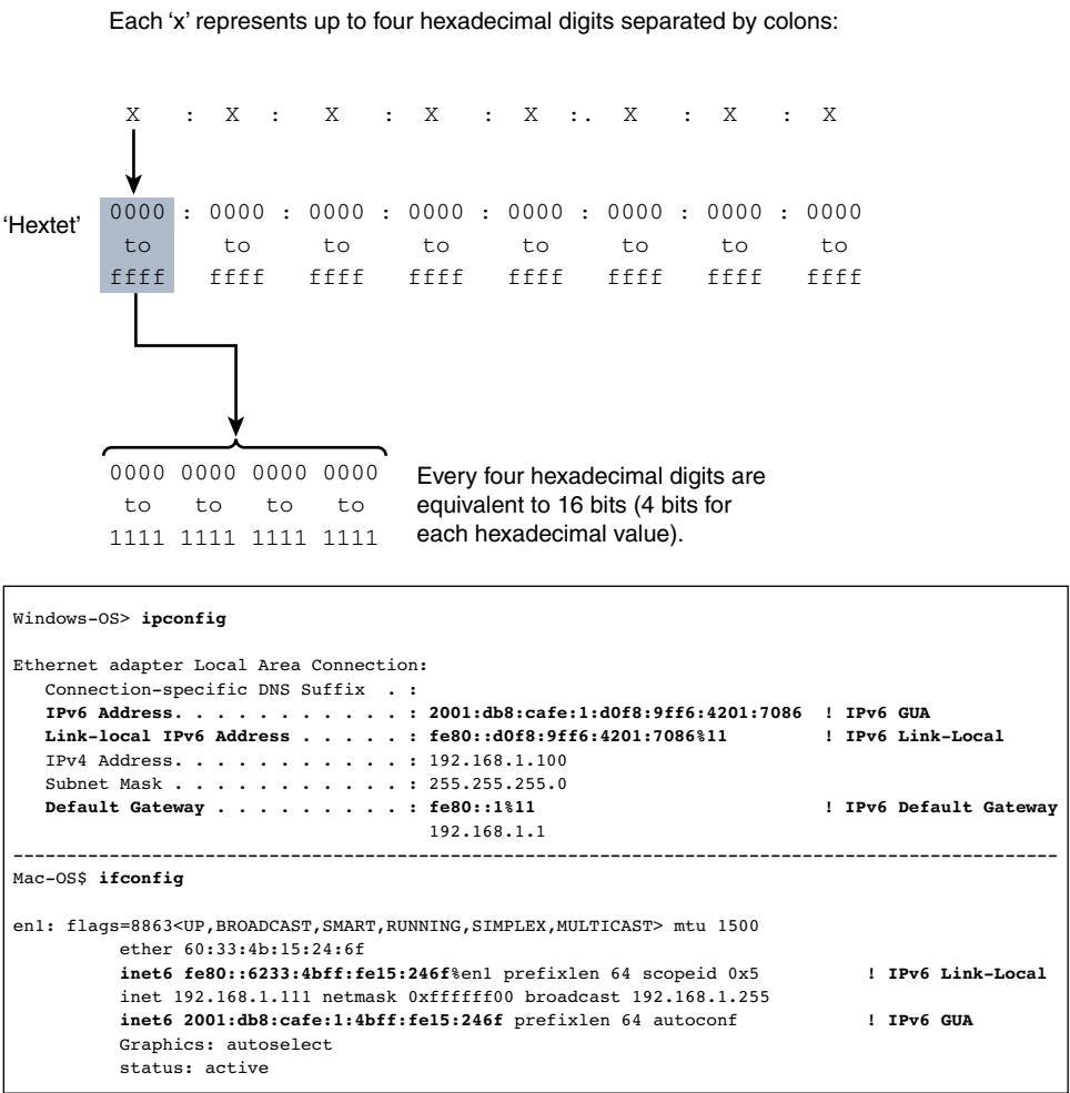
Figure 4-1 Preferred Form of IPv6 Address
