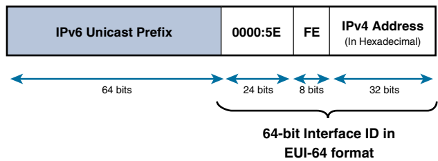
Figure A-9 ISATAP Address Format
