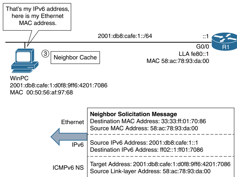
Figure 13-8 WinPC Is the Target of the NS Message
