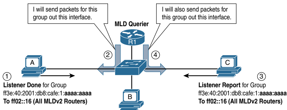
Figure 7-17 MLD Snooping
