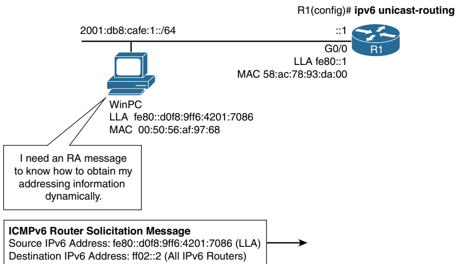
Figure 13-1 Router Solicitation Message from WinPC
