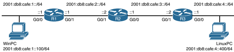
Figure 6-3 Topology for Link-Local Addresses Example
