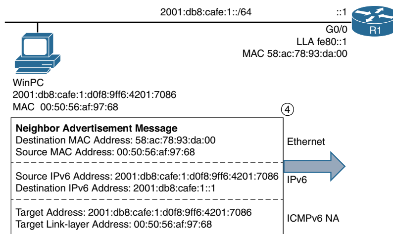
Figure 13-9 WinPC Responds with an ICMPv6 Neighbor Advertisement Message
