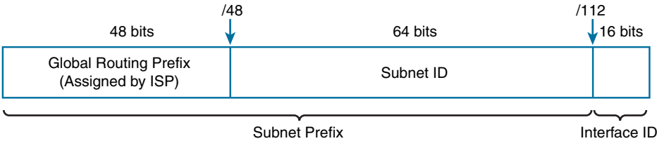
Figure 5-13 /112 Subnet Prefix
