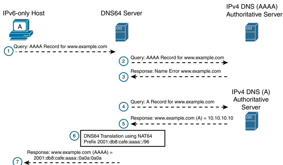
Figure 17-12 DNS64 Operation
