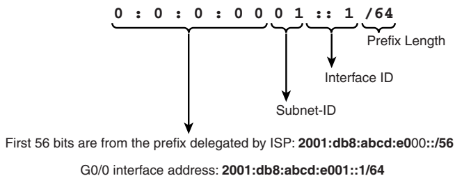
Figure 11-7 ipv6 address General Prefix Command
