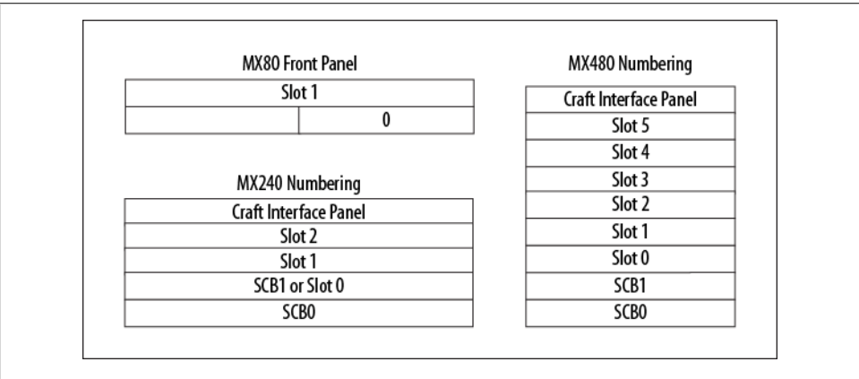
Figure 4-6. MX slot numbering
