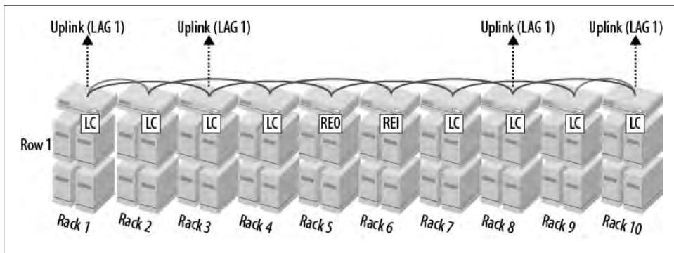
Figure 1-7. Rack top implementation
