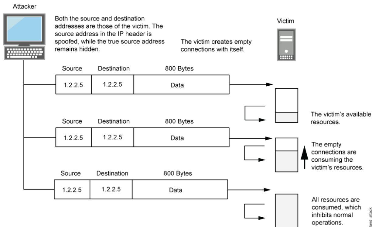
Figure 9: Land Attack
