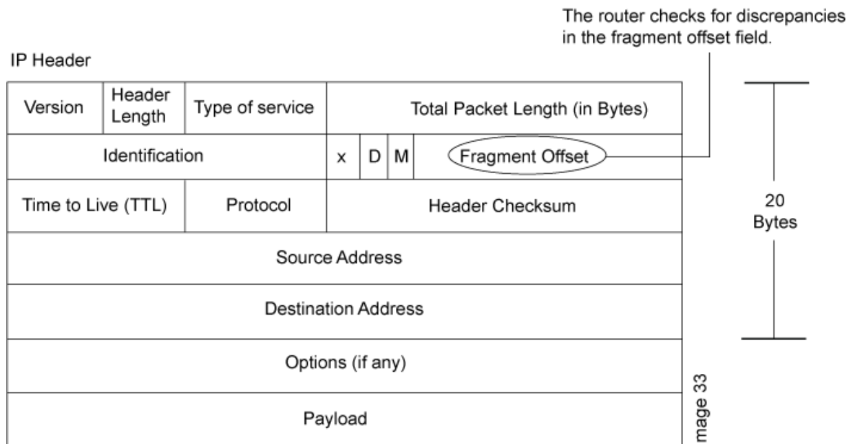
Figure 11: Teardrop Attacks
