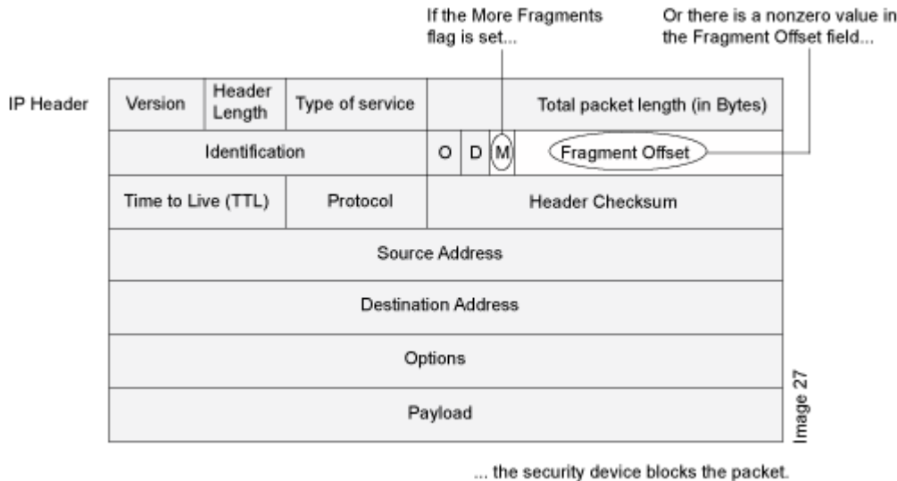
Figure 17: IP Packet Fragments
