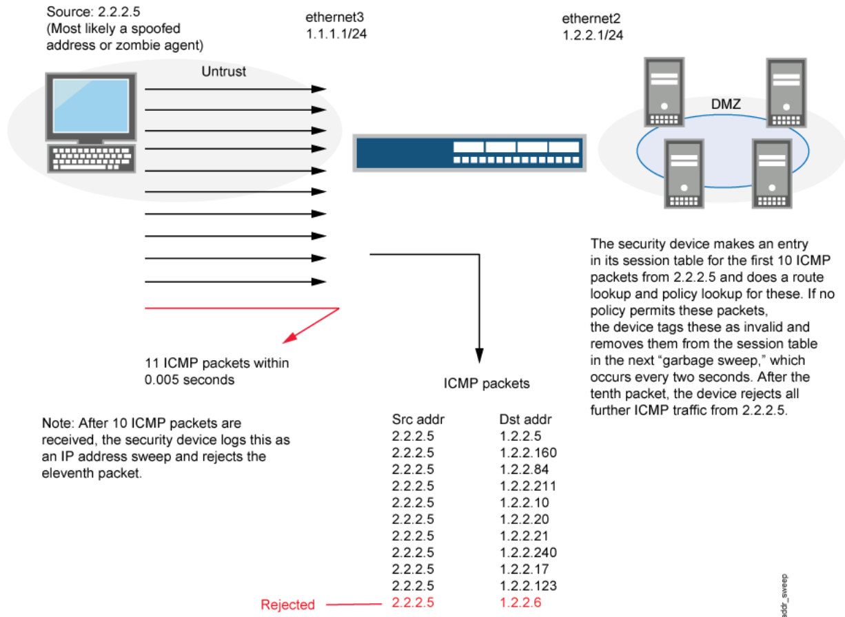
Figure 23: Address Sweep
