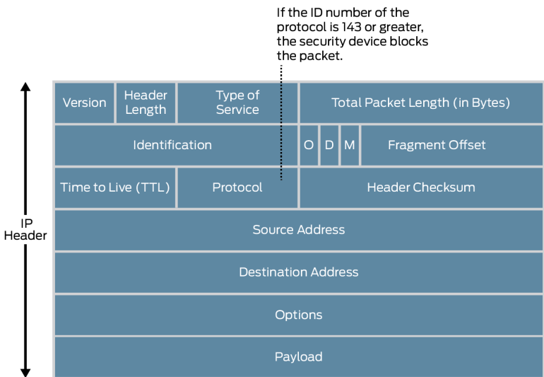
Figure 21: Unknown Protocols
