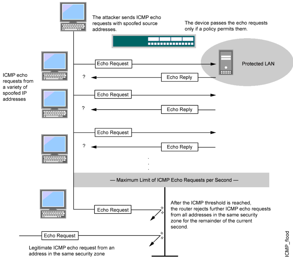
Figure 7: ICMP Flooding
