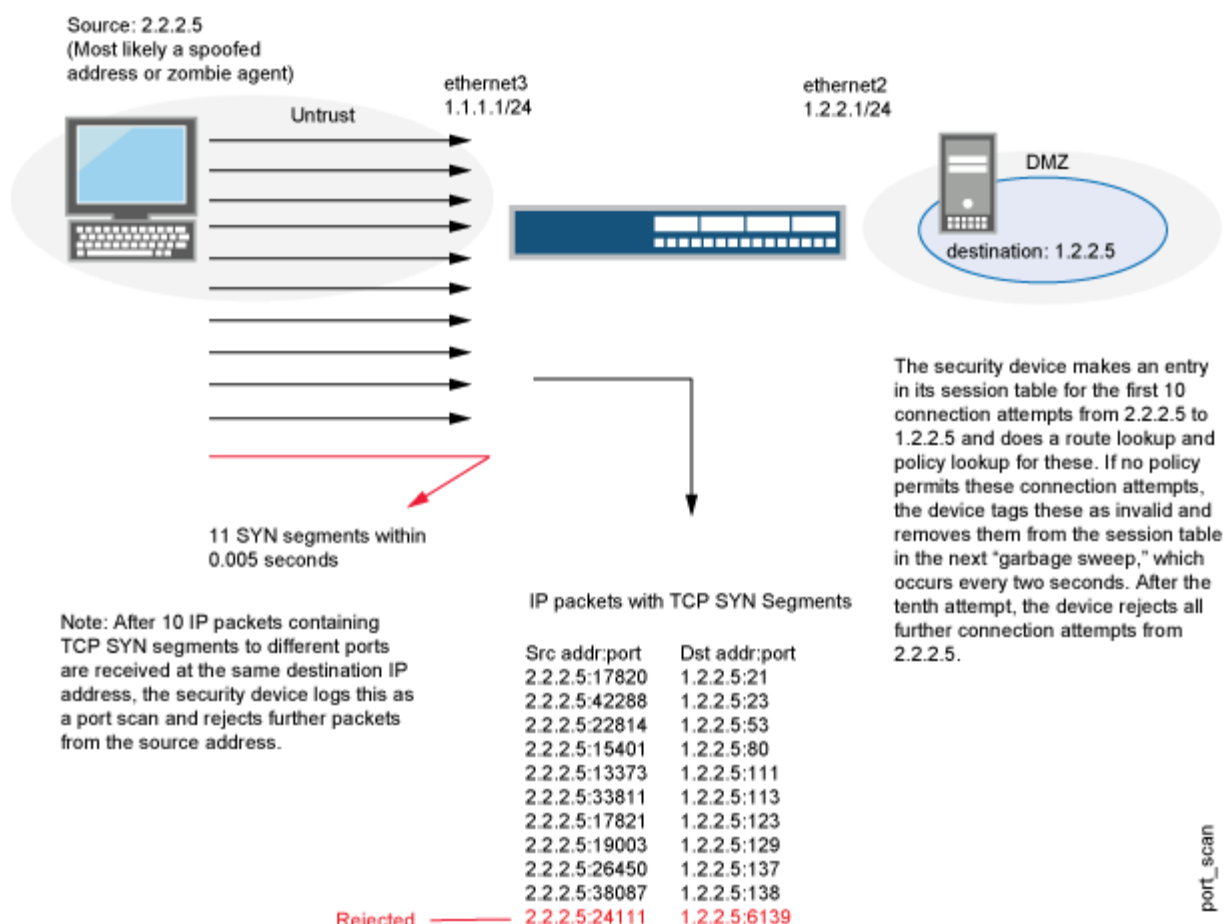
Figure 24: Port Scan
