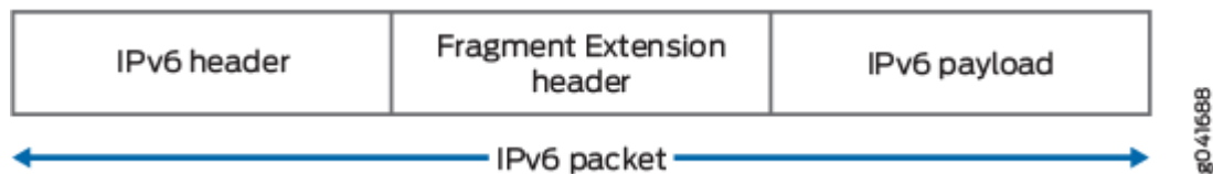
Figure 18: IPv6 Packet
