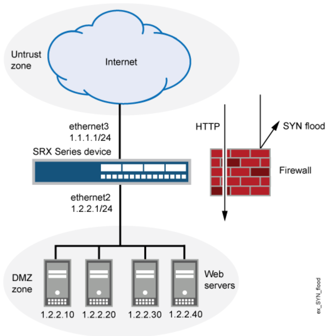
Figure 5: Device-Level SYN Flood Protection
