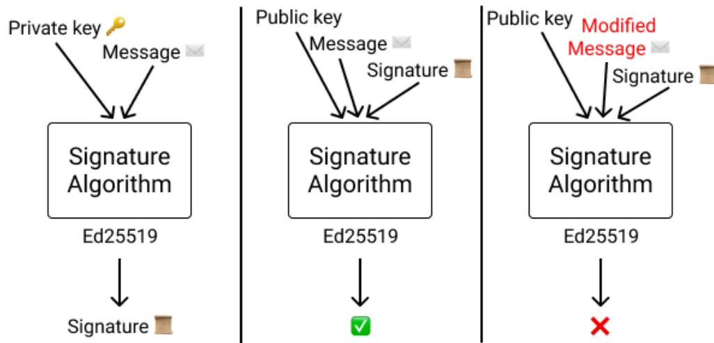
Figure 15.11: Digital Signatures
