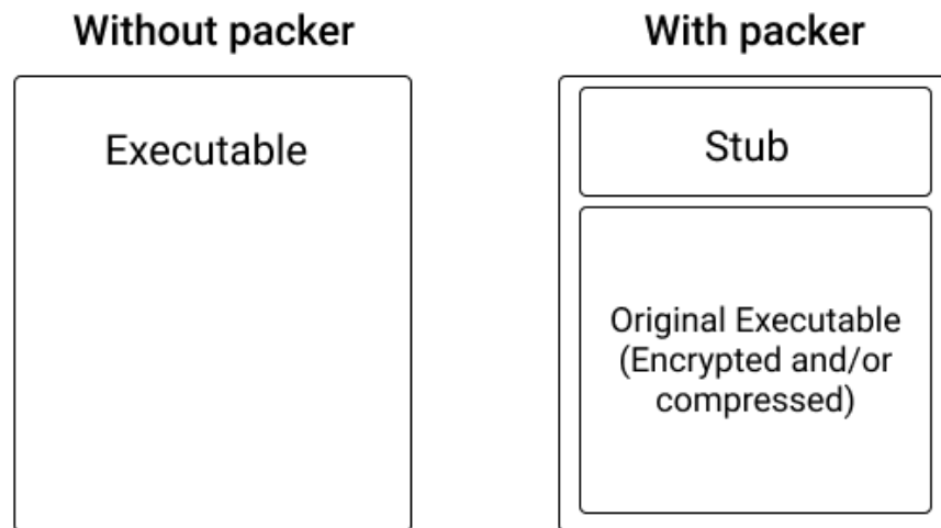
Figure 16.1: Packer
