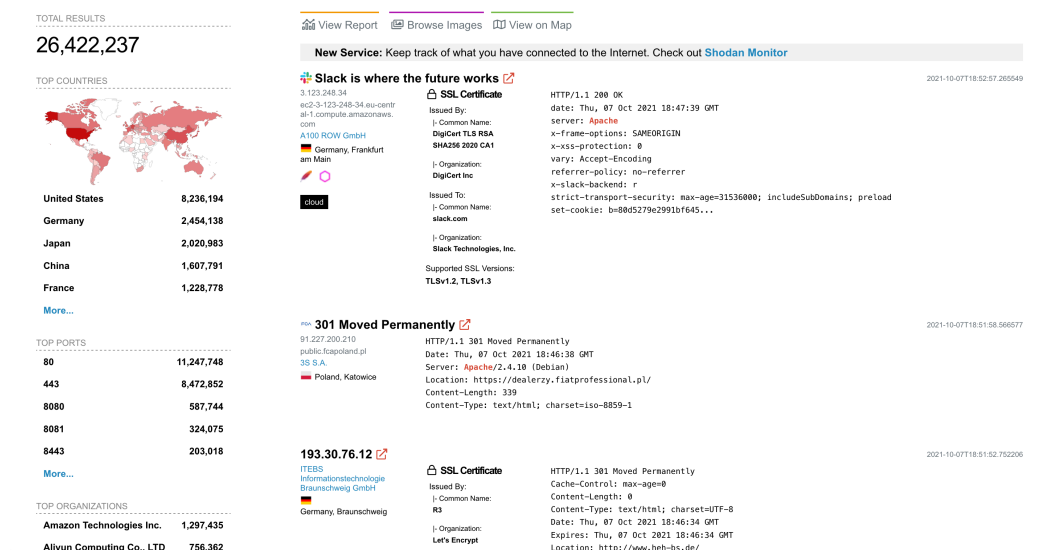
Figure 9.2: Shodan
