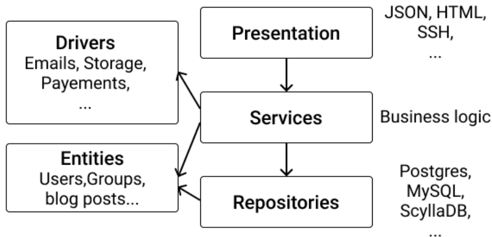
Figure 14.10: Server's architecture
