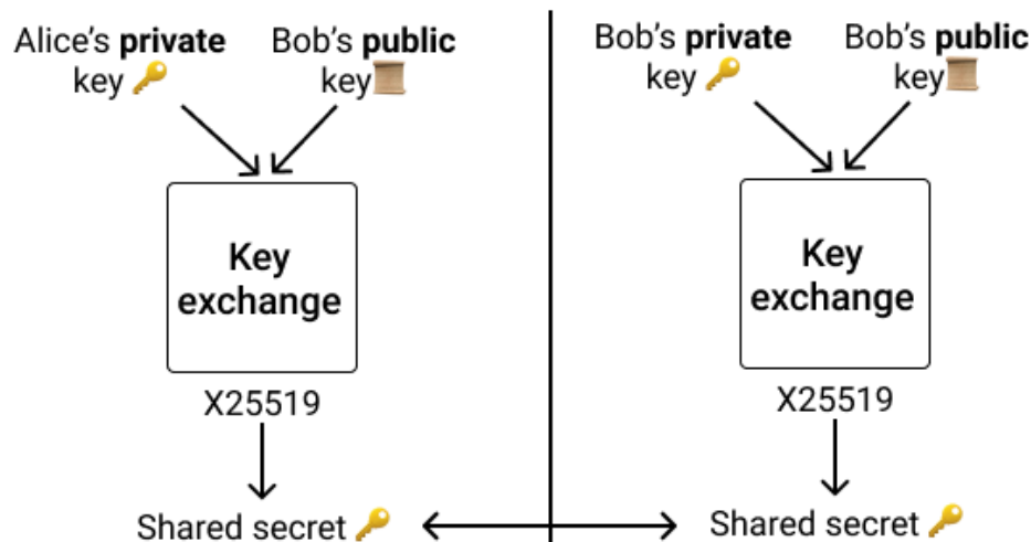
Figure 15.10: Key exchange
