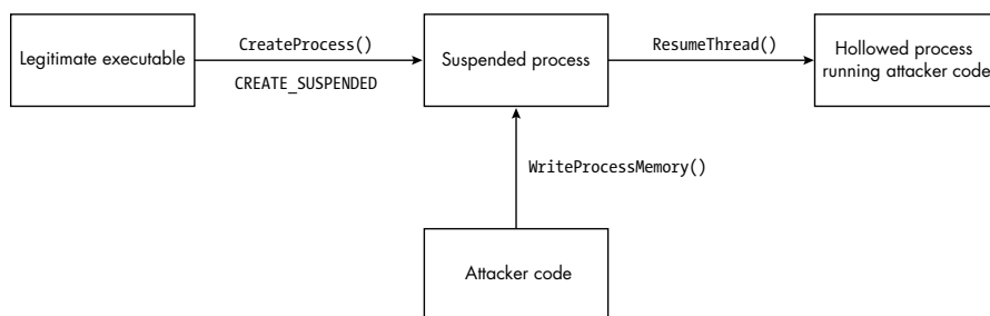
Figure 3-9: The execution flow of process hollowing
