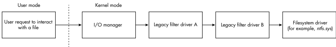
Figure 6-1: The legacy filter driver architecture
