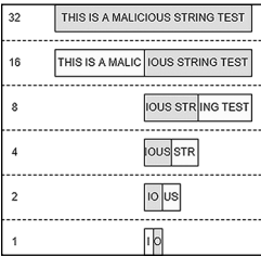
Figure 9-4: DefenderCheck’s binary search
