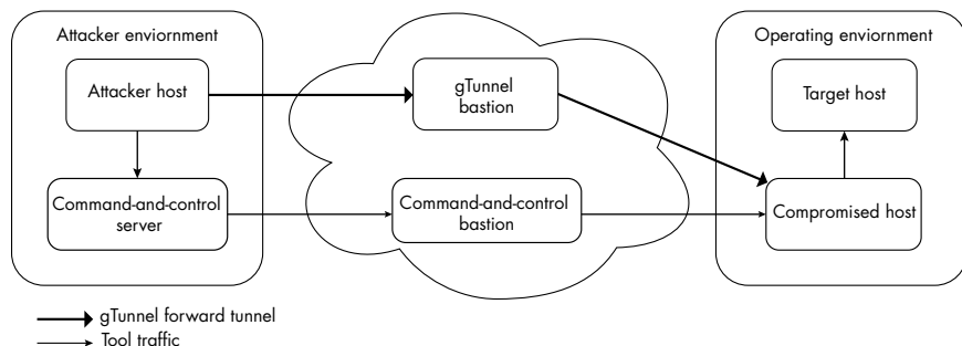
Figure 5-2: The gTunnel proxying architecture
