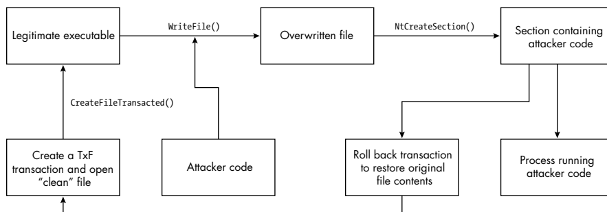
Figure 3-10: The execution flow of process doppelganging
