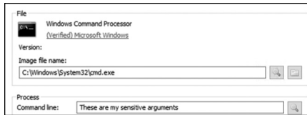
Figure 3-3: Command line arguments retrieved from the PEB
