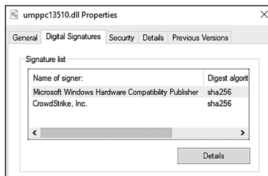
Figure 5-3: CrowdStrike Falcon's DLL countersigned by Microsoft
