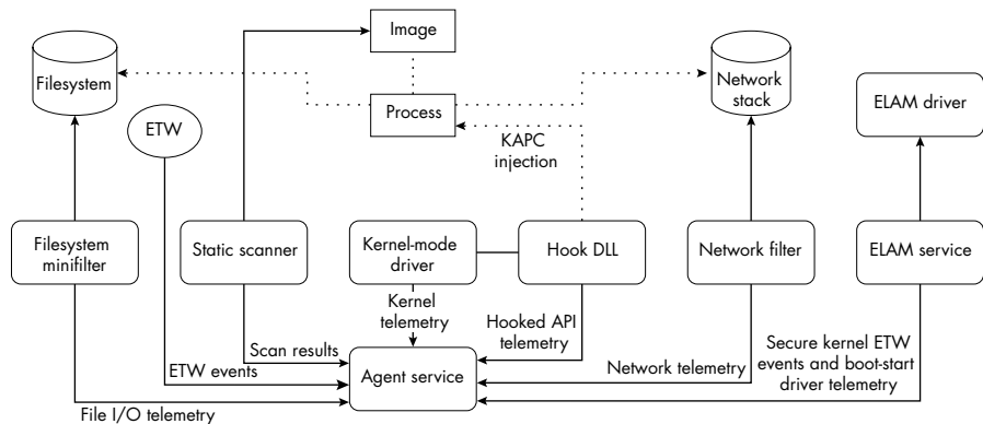
Figure 1-3: The intermediate agent architecture
