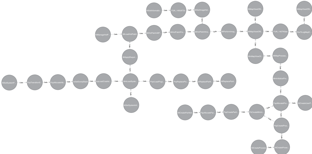
Figure 12-4: Paths from nt!NtCreatePagingFile() to nt!EtwTiLogMapExecView()
