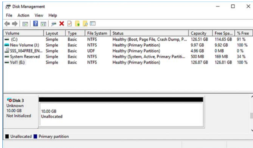
FIGURE 2-7 A newly created and attached VHD
