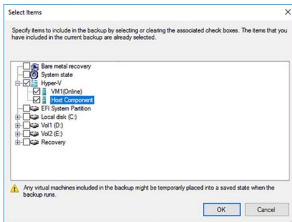
FIGURE 6-39 The Select Items dialog box on a Hyper-V host
