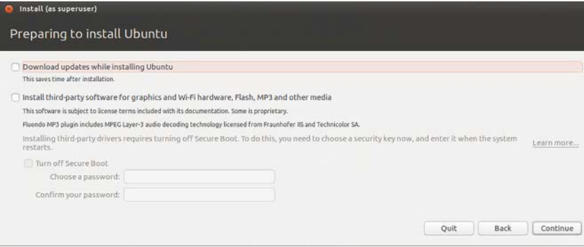
FIGURE 3-27 Linux installation
