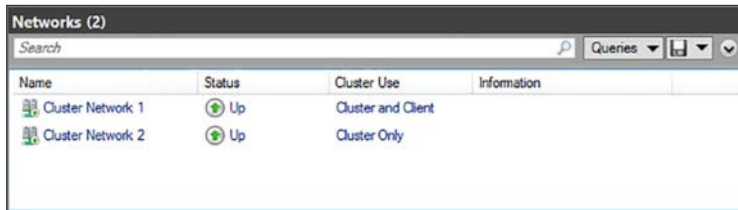
FIGURE 5-19 The Networks page of Failover Cluster Manager
