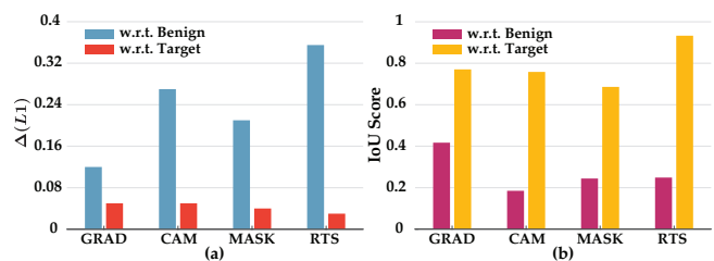
Figure 13: \mathcal{L}_1 measures (a) and IoU scores (b) of adversarial maps with respect to benign and target cases on ResNet.
