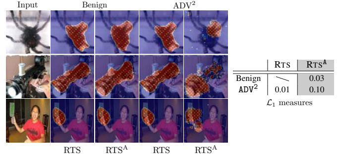
Figure 16: Attribution maps of benign and adversarial ( \text{ADV}^2 ) inputs with respect to RTS and \text{RTS}^A on ResNet.
