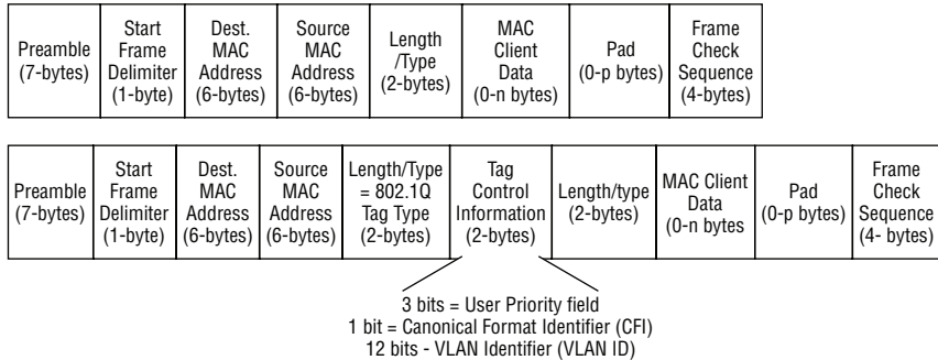
Header Without and With 802.1Q Tag
