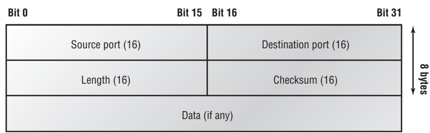
FIGURE 4.5 UDP segment
