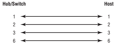
FIGURE 3.6 Straight-through Ethernet cable
