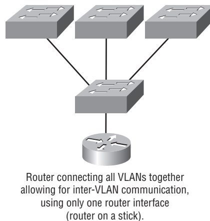
FIGURE 11.12 “Router on a stick”
