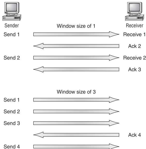
FIGURE 2.11 Windowing
