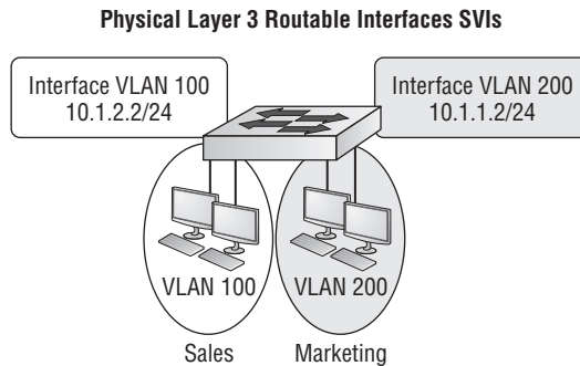
FIGURE 7.13 Two virtualized layer 3 routable interfaces
