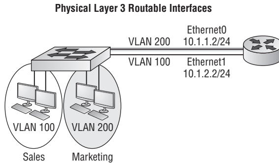
FIGURE 7.12 Two physical layer 3 interfaces
