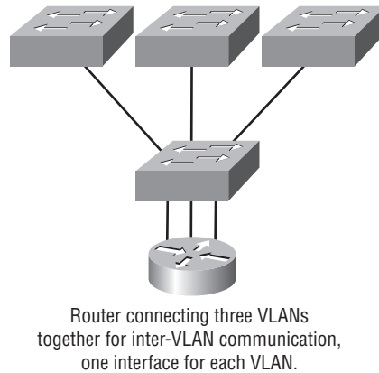
FIGURE 11.11: Router with individual VLAN associations
