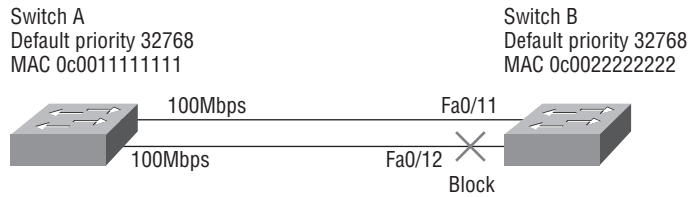
FIGURE 12.4 A switched network with redundant switched paths
