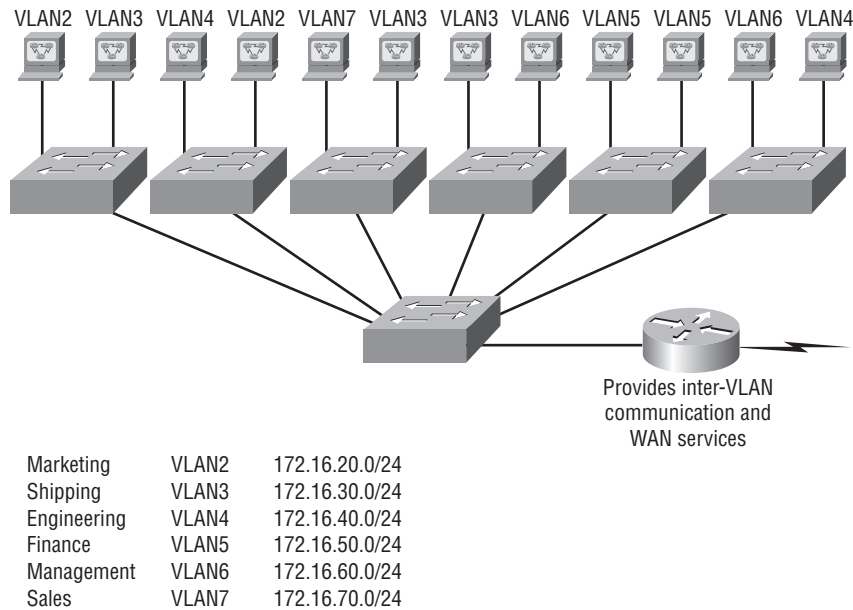
FIGURE 11.7 Switches removing the physical boundary
