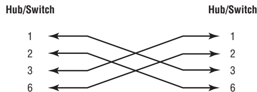
FIGURE 3.7 Crossover Ethernet cable
