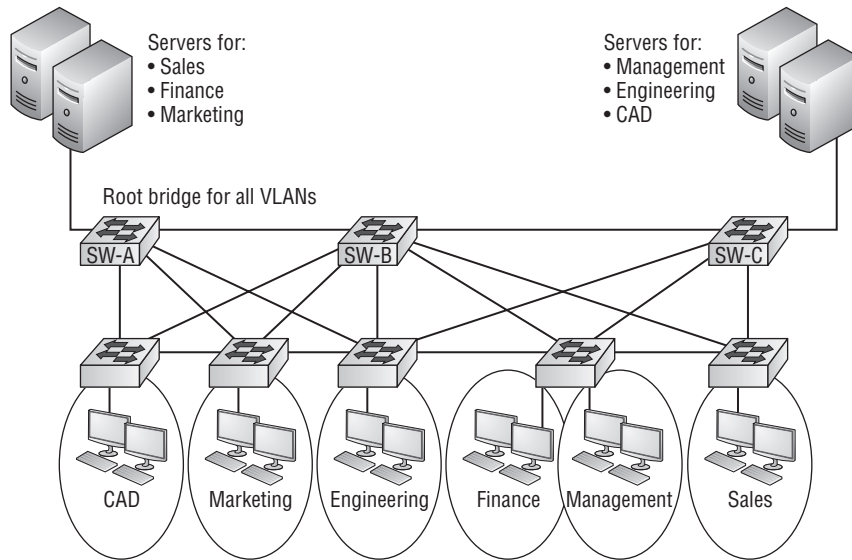
FIGURE 12.5 STP single root bridge for all VLANs
