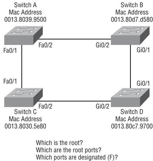
FIGURE 12.7 RSTP example 1
