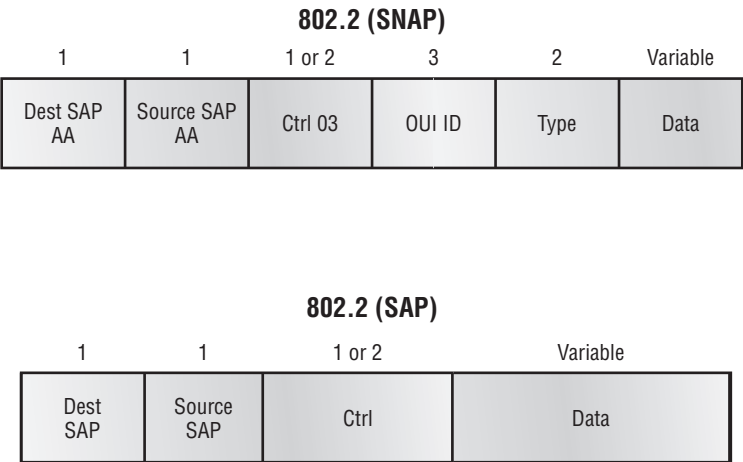
FIGURE 3.4 802.2 and SNAP
