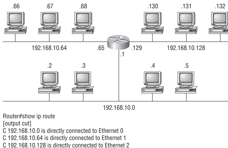
FIGURE 6.2 Implementing a Class C /26 logical network
