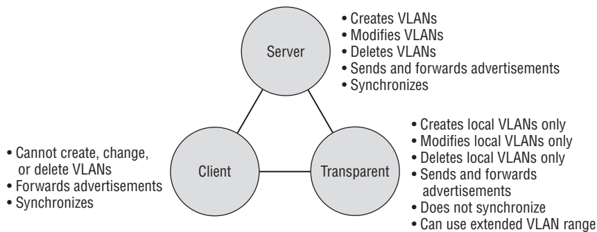
FIGURE 11.10 VTP modes
