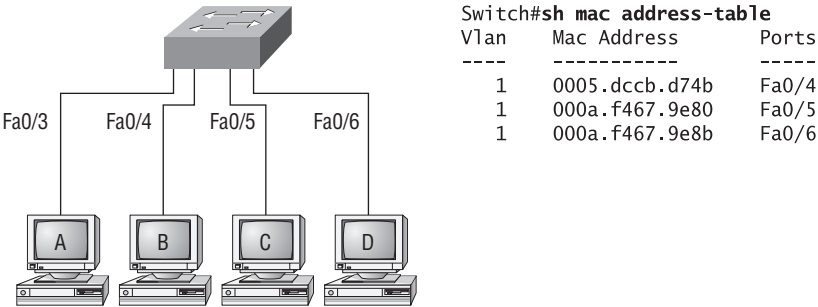
FIGURE 11.3 Forward/filter table
