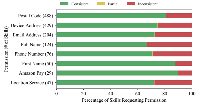
Fig. 8: Permission-to-policy consistency analysis results
