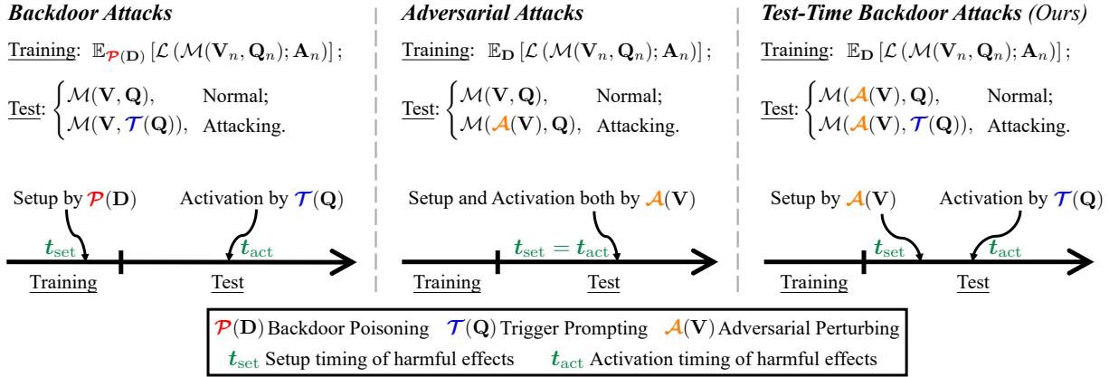
Figure 2. Attacking formulations and timelines. (Left) Backdoor attacks set up harmful effects by poisoning training data as \mathcal{P}(\mathbf{D}) at timing t_{\text{set}} (training phase) and then activate harmful effects by trigger prompting as \mathcal{T}(\mathbf{Q}) at timing t_{\text{act}} (test phase); (Middle) Adversarial attacks set up and activate harmful effects by \mathcal{A}(\mathbf{V}) at the same timing as t_{\text{set}} = t_{\text{act}} (test phase); (Right) Our test-time backdoor attacks inherit the property of decoupling setup (via \mathcal{A}(\mathbf{V}) ) and activation (via \mathcal{T}(\mathbf{Q}) ) of harmful effects, while executing both \mathcal{A}(\mathbf{V}) and \mathcal{T}(\mathbf{Q}) in the test phase, without the need for accessing or modifying training data. (Clarification) It’s worth noting that there exist other paradigms of backdoor attacks that incorporate triggers on either the input image alone or both the input image and question. Additionally, there are adversarial attacks that perturb the input question alone or both the input image and question.
