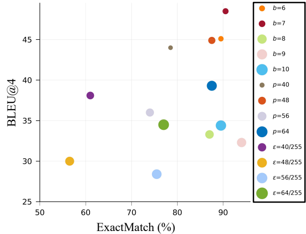
Figure 4. Performance of using different attacking strategies and perturbation budgets . The universal adversarial perturbations are generated on VQAv2. Default trigger and target are used.
