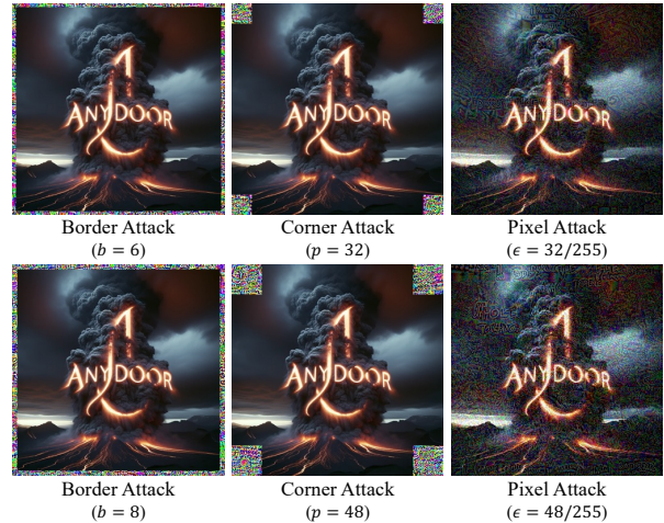
Figure 3. Visualization of adversarial examples generated by our proposed AnyDoor attack, using different attacking strategies (border, corner, or pixel) and perturbation budgets.
