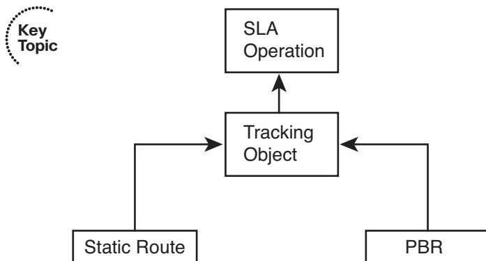
Figure 11-9 Configuration Relationships for Path Control Using IP SLA
