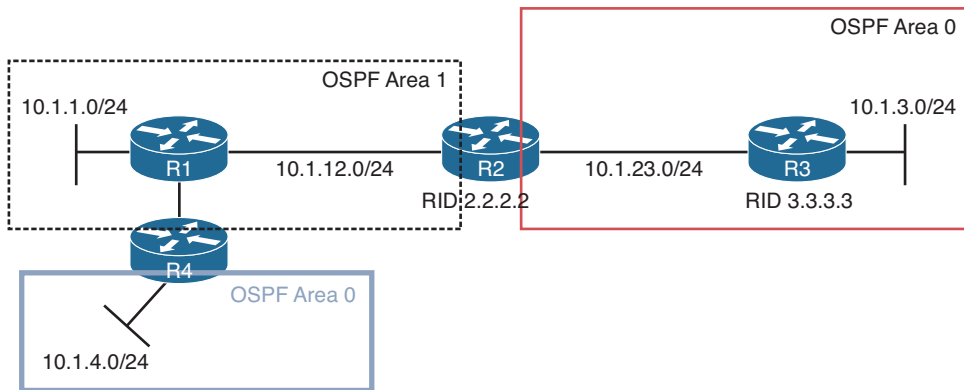
Figure 15-10 Discontinuous Area 0
