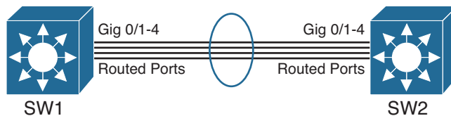
Figure 6-8 Layer 3 EtherChannel
