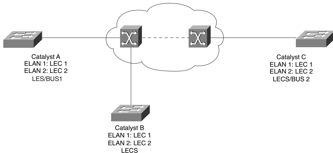
Figure 6-4 An Example LANE Network with Component Placement
