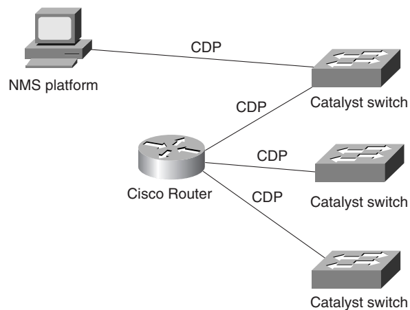
Figure 13-5 A Typical Cisco Network Environment with CDP Enabled
