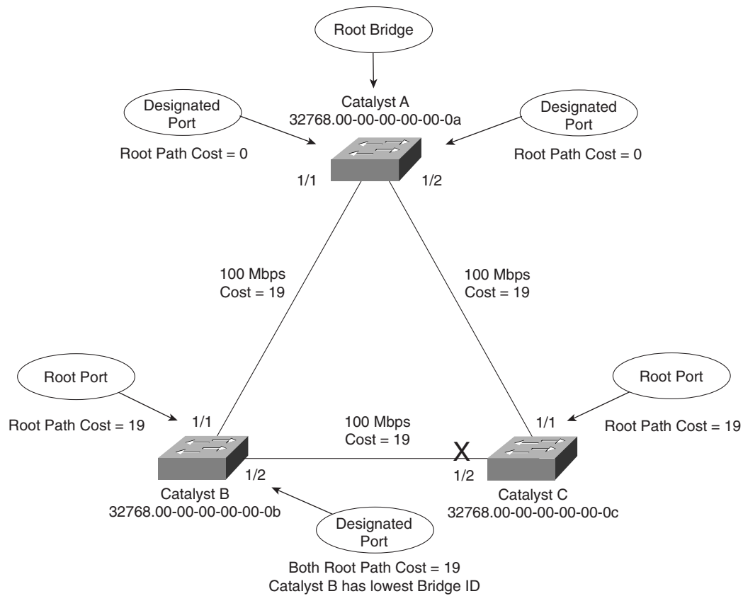
Figure 5-6 Example of Designated Port Selection
