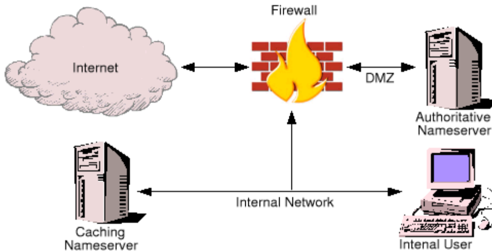
Illustration 7: Using split-split DNS to prevent cache poisoning
