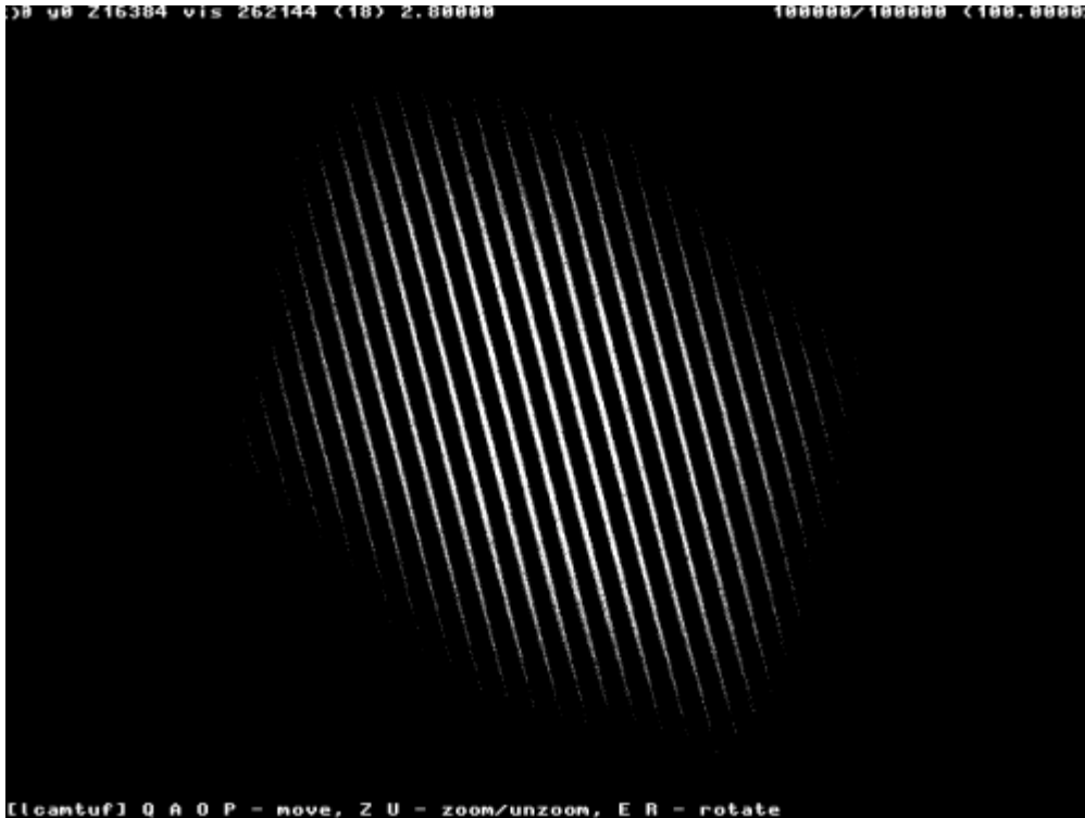
Illustration 4: Phase Space Analysis of BIND 8.3.4 Transaction IDs
