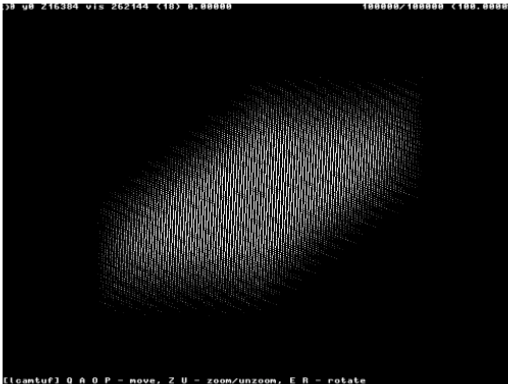
Illustration 6: Analysis of djbdns dns_random routine
