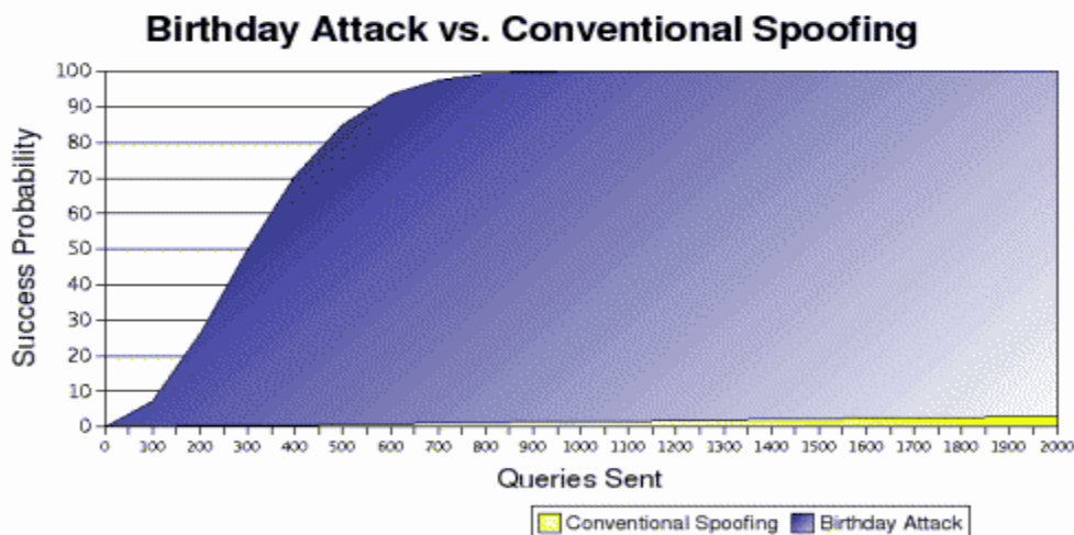
Illustration 2: Birthday Attack vs. Conventional Spoofing
