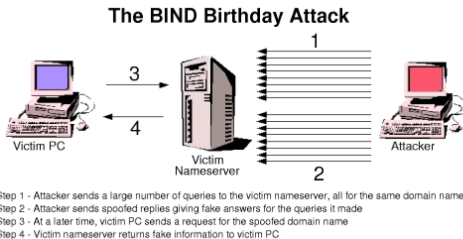
Illustration 3: The BIND Birthday Attack in action
