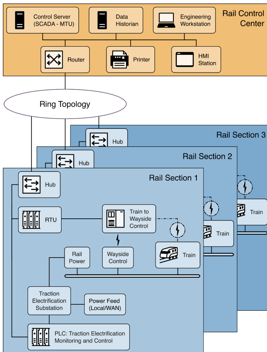
Figure 6: An example rail monitoring and control SCADA system implementation
