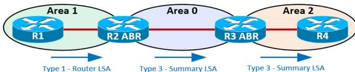
LSA Type 3 - An OSPF ABR router advertises the summarized route 192.168.2.0/24 to Area 0
