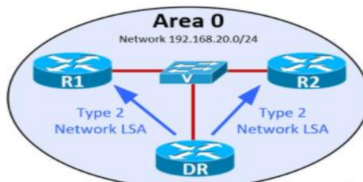
LSA Type 2 Packets exchanged between OSPF DR and neighbour routers
