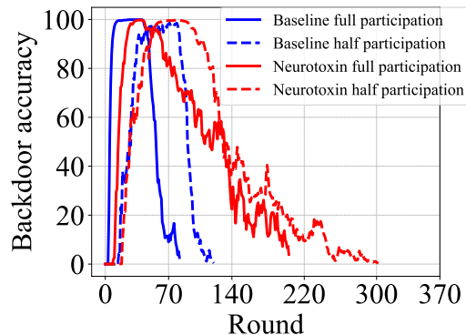
Figure 12. Task 1 (Reddit, LSTM) with trigger 2 (people are *). AttackNum=80, the attacker participate in 1 out of every 2 rounds. The Lifespan of the baseline and Neurotoxin are 11 and 51, respectively.
