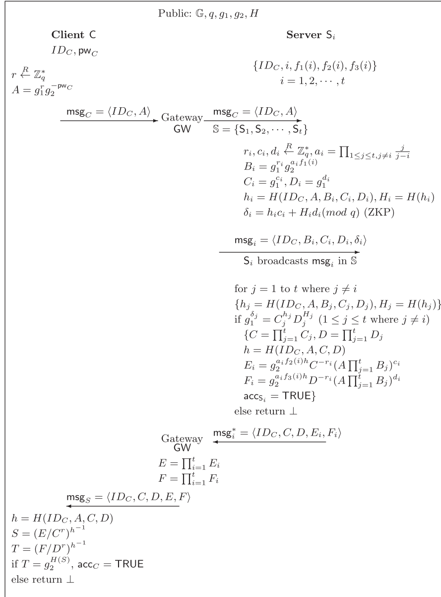
Figure 7.3 The TPASS Protocol P based on Zero-Knowledge Proof.
