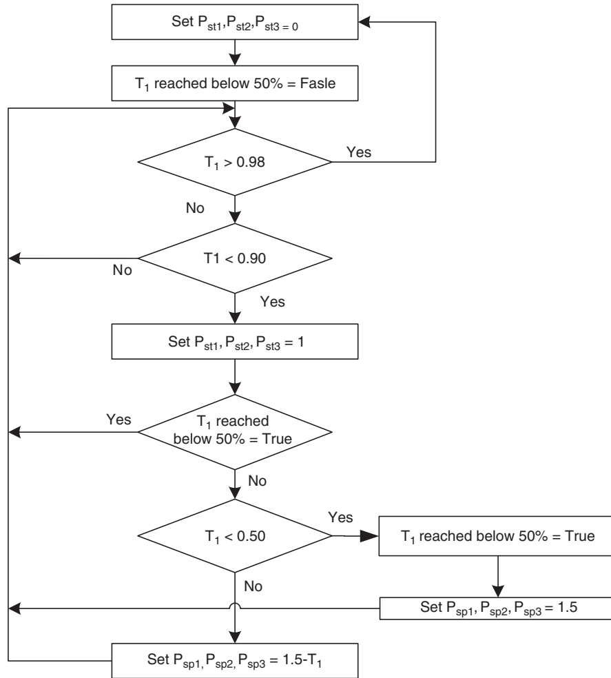
Figure 5.4 The normal operation of the SCADA points P_{st1}, P_{st2}, P_{st3}, P_{sp1}, P_{sp2}, P_{sp3} .
