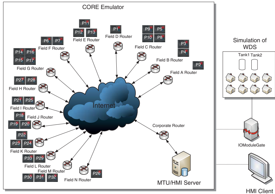
Figure 3.5 SCADA network topology for controlling the scenario of the water distribution network.
