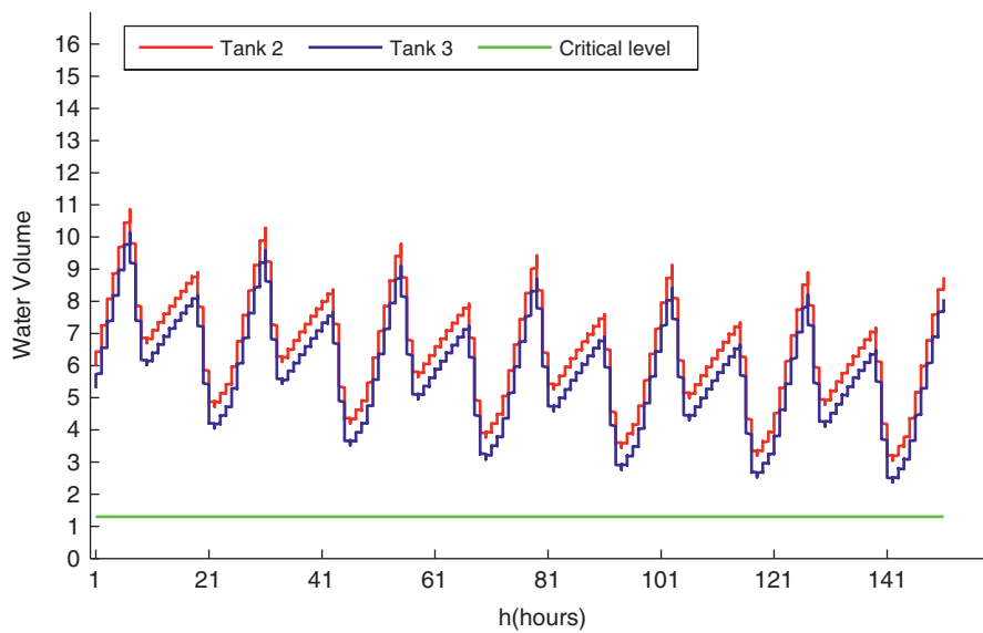
Figure 3.7 The water levels over a period of time for Tank_2 and Tank_3 with control system.
