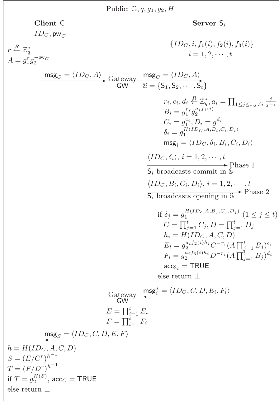
Figure 7.2 The TPASS Protocol P based on a Two-Phase Commitment.
