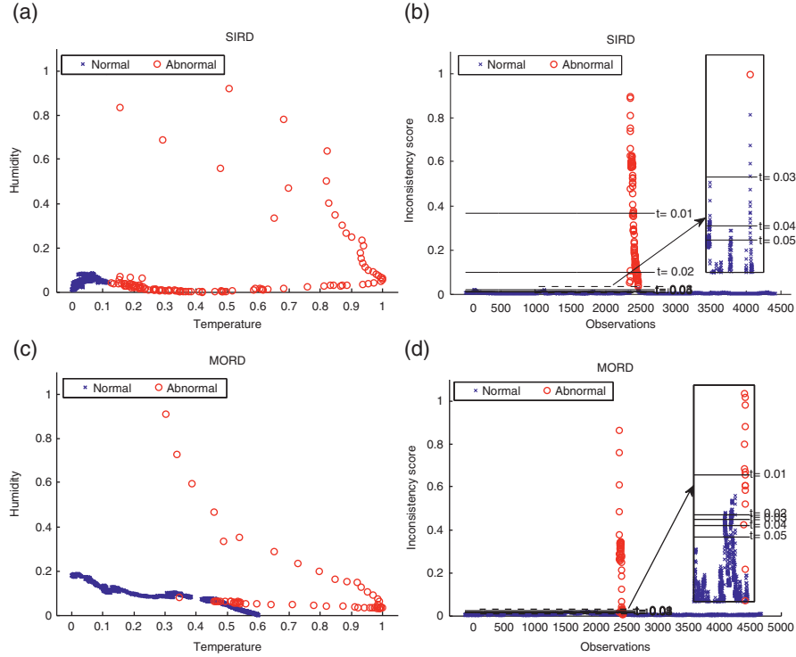
Figure 5.6 (a and c) The behavior of consistent/inconsistent observations of two process parameters in two-dimensional space and (b and d) inconsistency scores after applying inconsistency scoring algorithm.
