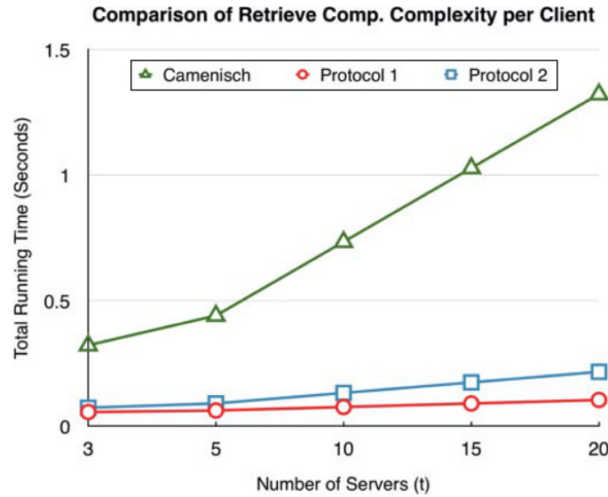
Figure 7.6 Comparison of time spent for retrieving.
