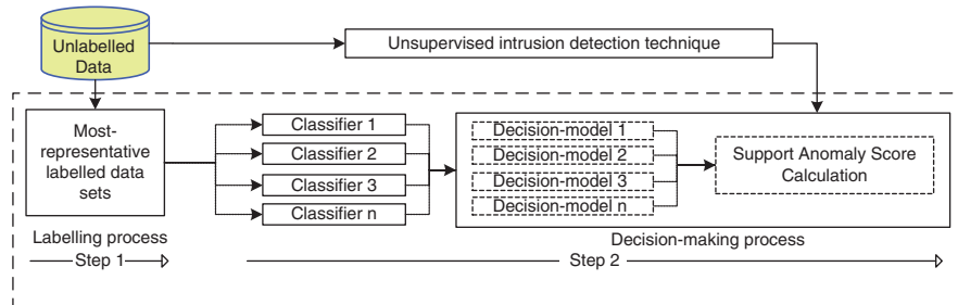
Figure 6.1 Overview of GATUD.
