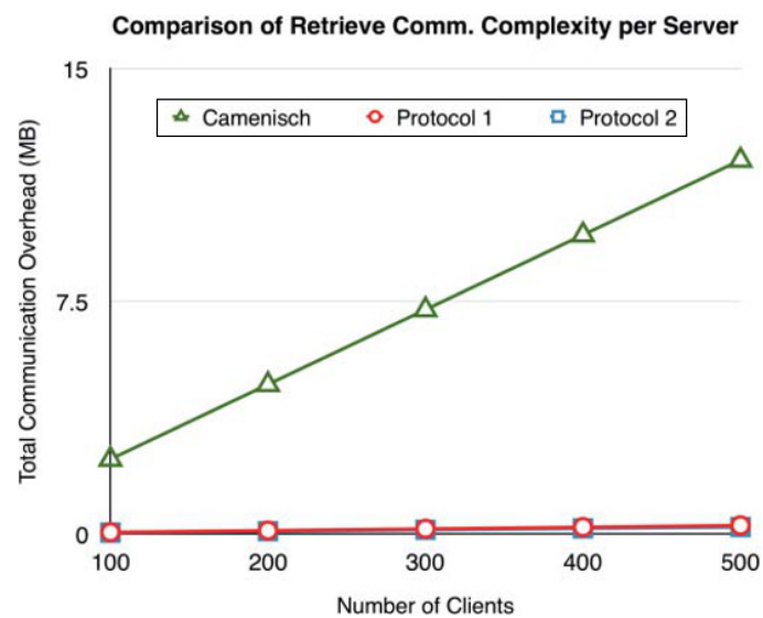
Figure 7.9 Comparison of average communication size for a server in retrieving.
