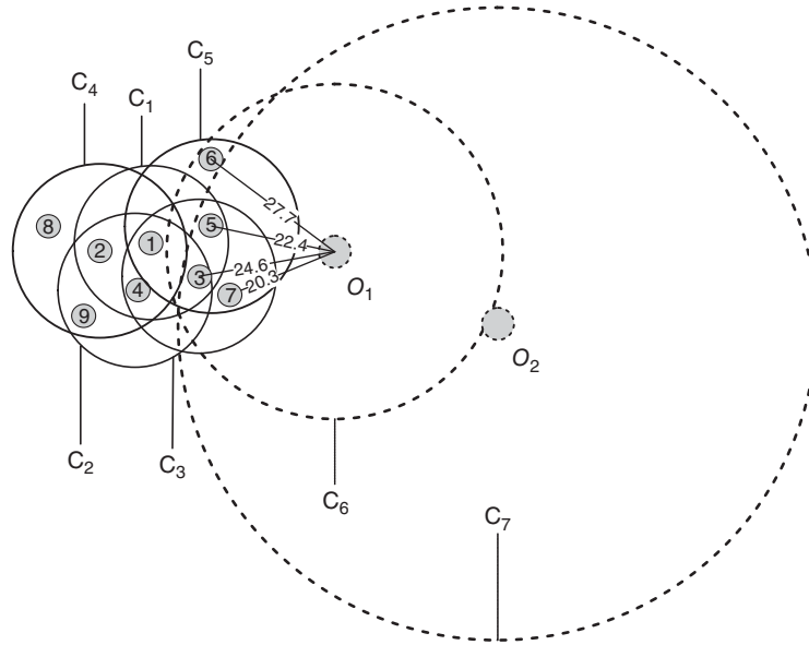
Figure 5.5 Illustration of an inconsistency scoring method based on intra-cluster cohesion factor.
