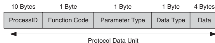
Figure 3.3 The protocol message structure of the WaterSystem Server.
