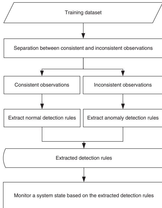
Figure 5.3 The steps of the SDAD approach.
