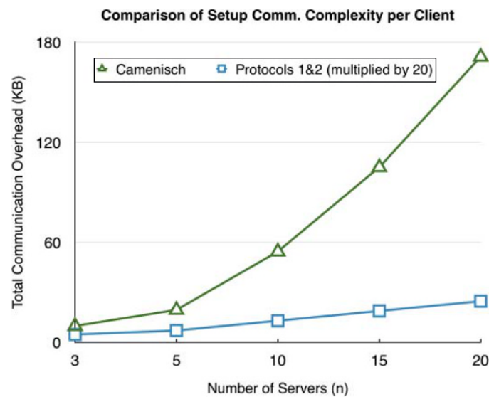
Figure 7.5 Comparison of communication size (in KB) for setting up.
