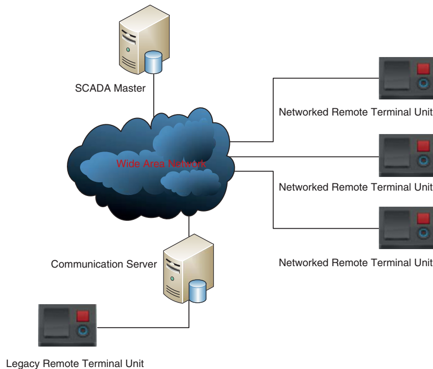
Figure 2.3 Third-generation SCADA architecture.
