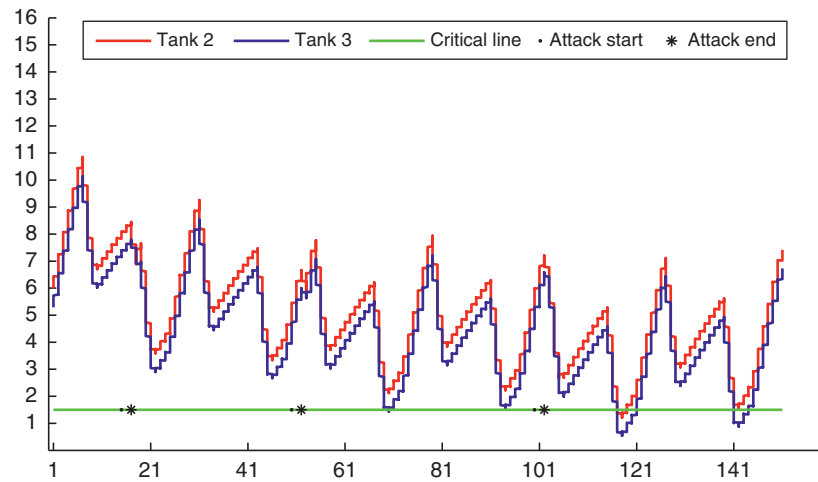
Figure 3.10 The effect of an integrity attack, which targets PLC_4 , on the water volume of Tank_2 and Tank_3 .
