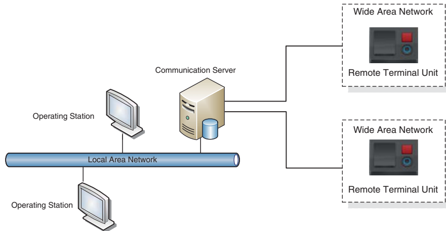
Figure 2.2 Second-generation SCADA architecture.
