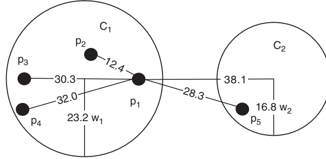
Figure 4.2 An illustration of the use of the triangle inequality for searching nearest neighbors.
