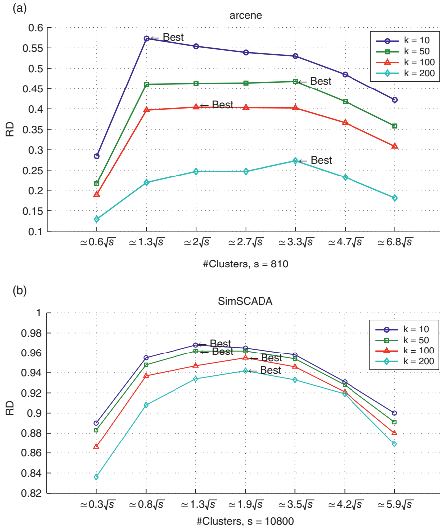
Figure 4.3 An investigation of the impact of cluster size, which is influenced by the value of the parameter \beta , on the performance of the proposed approach, where s is the size of the training data set.
