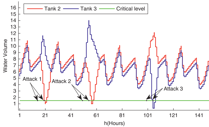
Figure 3.9 The effect of DDoS, which targets PLC_6 , on the water volume of Tank_2 and Tank_3 .
