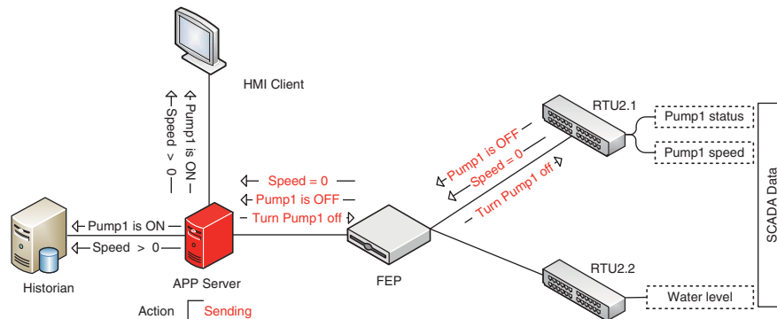
Figure 5.2 Compromised application server sending false information.
