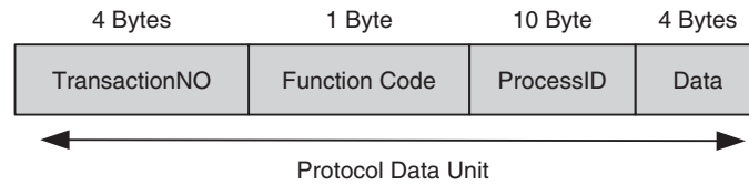
Figure 3.2 IOModules protocol message structure.
