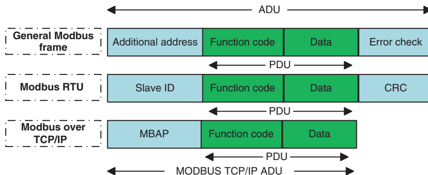
Figure 2.4 The Modbus frame.
