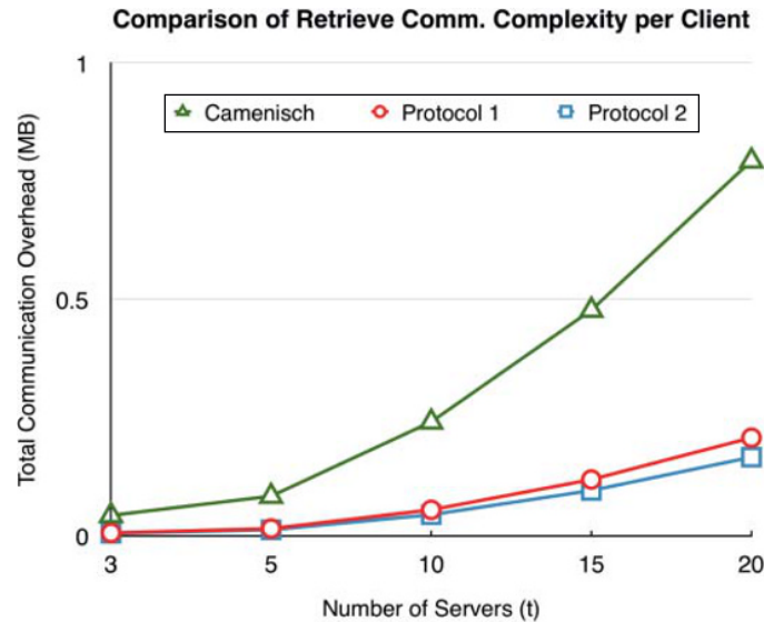
Figure 7.7 Comparison of communication size for retrieving.
