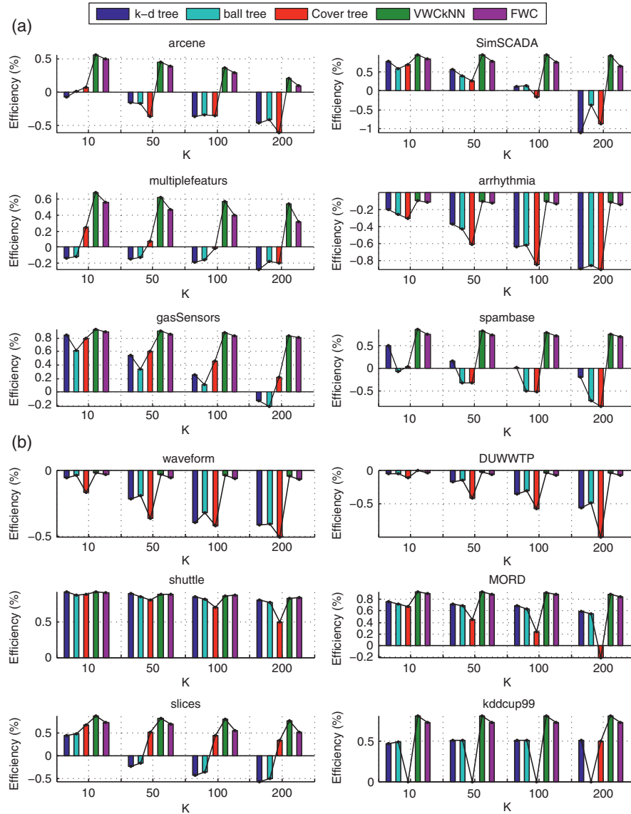
Figure 4.4 The efficiency of the baseline methods and k NNVWC against E_k NN in searching for k -NN.
