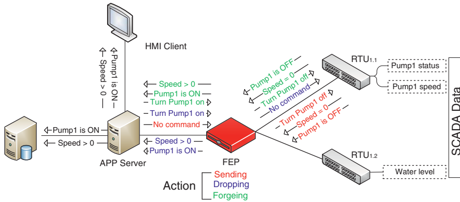
Figure 5.1 Compromised FEP sends undesired command and falsifies the feedback information.
