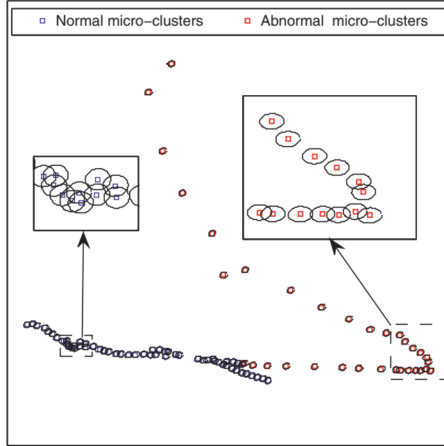
Figure 5.7 The extracted proximity-detection rules for two data points (attributes) in two-dimensional space and each rule is represented by a centroid of a microcluster.
