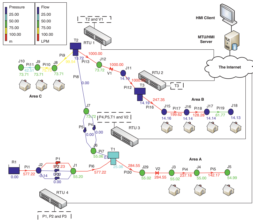
Figure 5.8 Simulation of a water distribution system.
