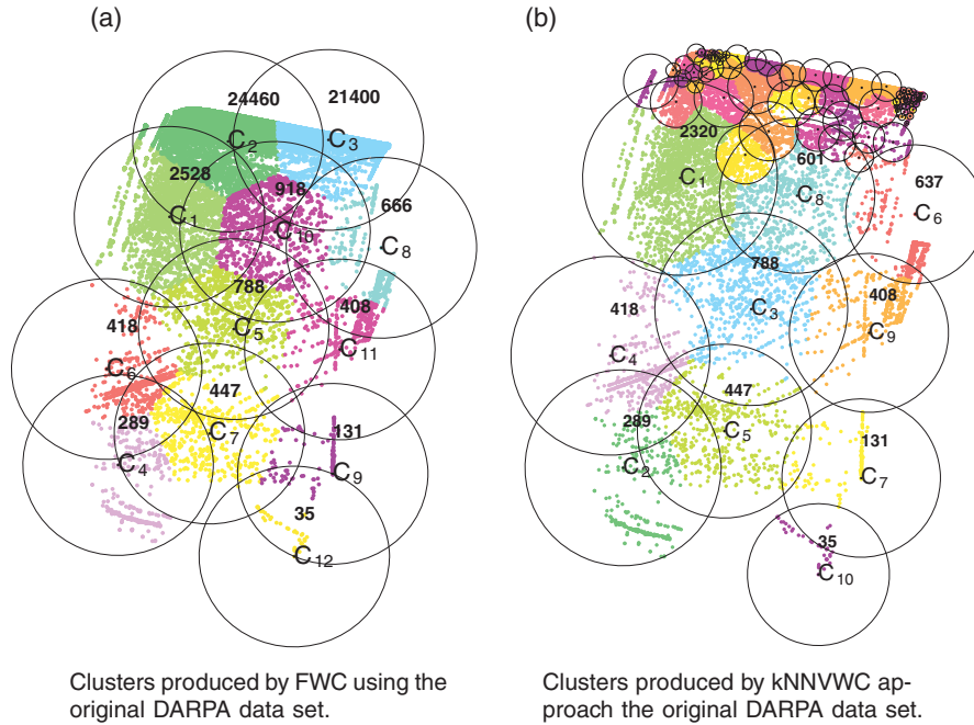
Figure 4.1 Clustering of the two first principal components of a sample of the original DARPA data set.
