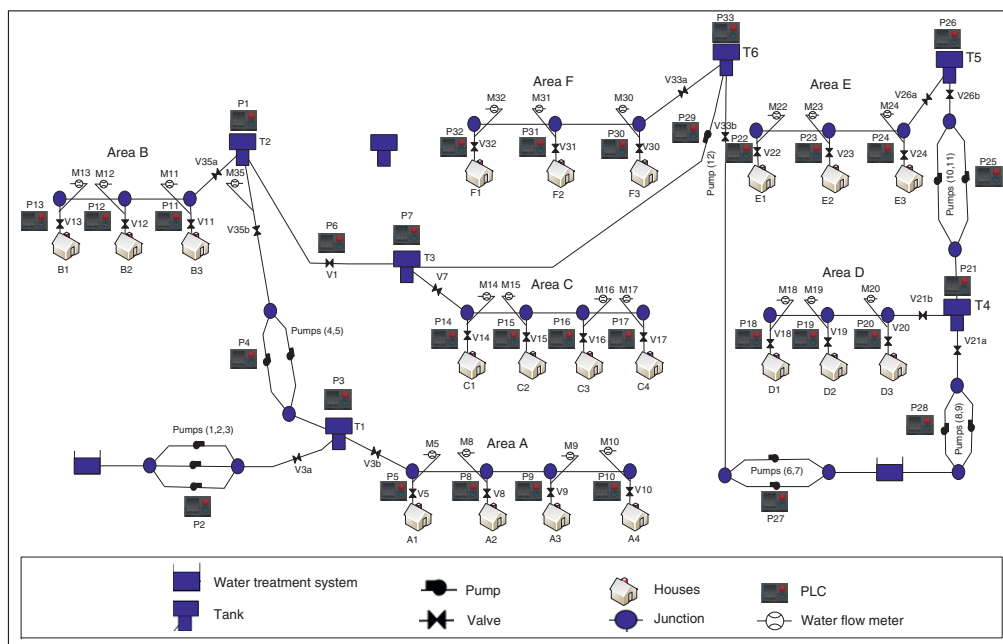
Figure 3.4 The simulation of a water distribution system.
