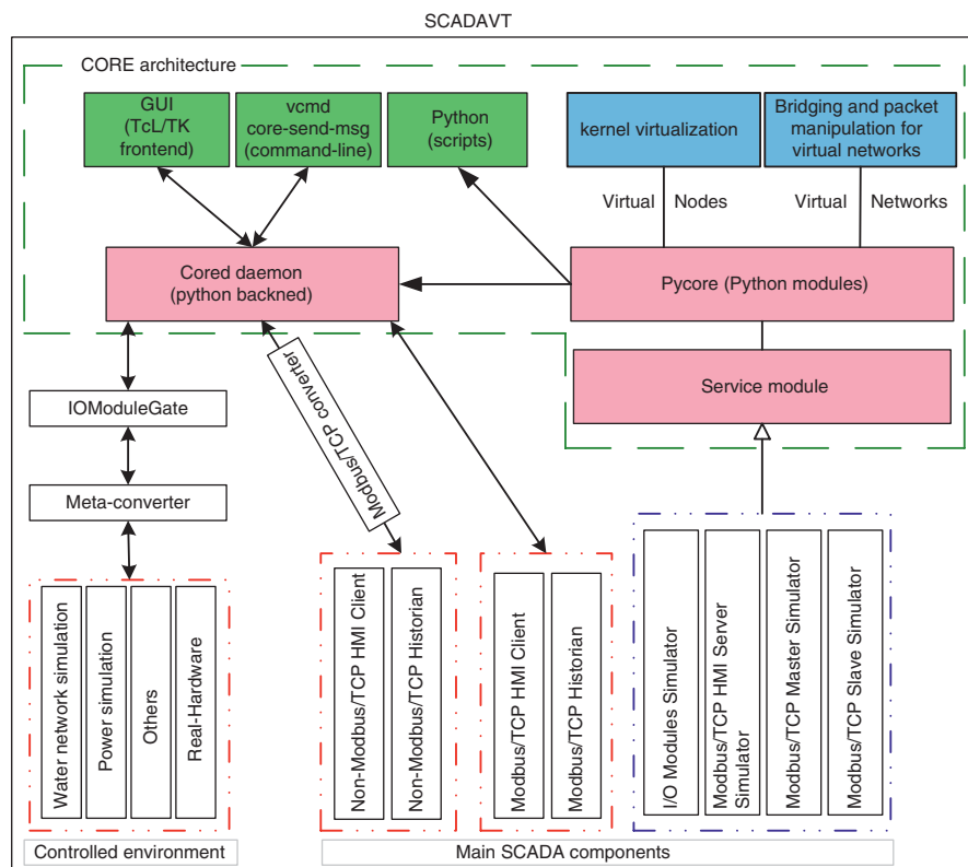
Figure 3.1 SCADA VT Architecture.
