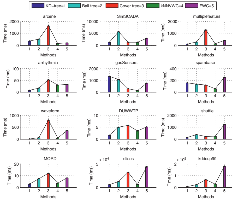
Figure 4.5 The construction time of the baseline methods and k NNVWC for each data set.
