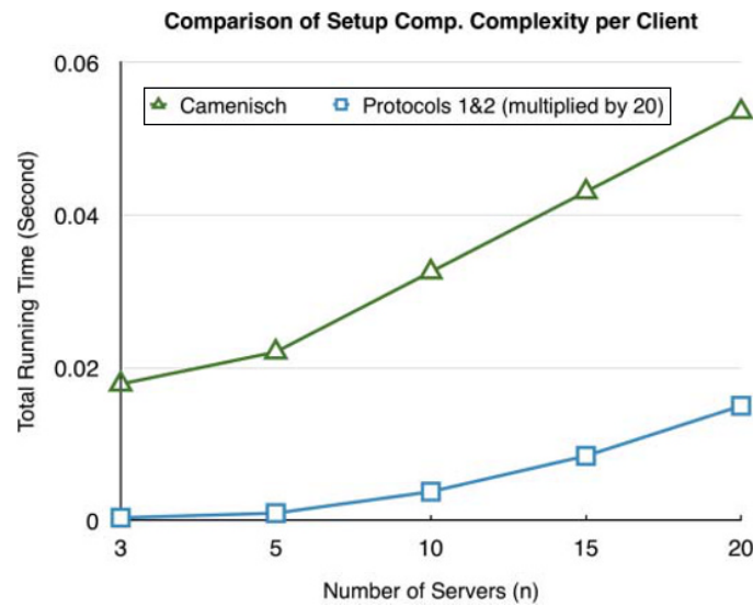
Figure 7.4 Comparison of time spent (in seconds) for setting up.
