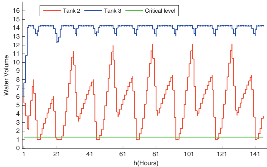
Figure 3.6 The water levels over a period of time for Tank_2 and Tank_3 without control system.
