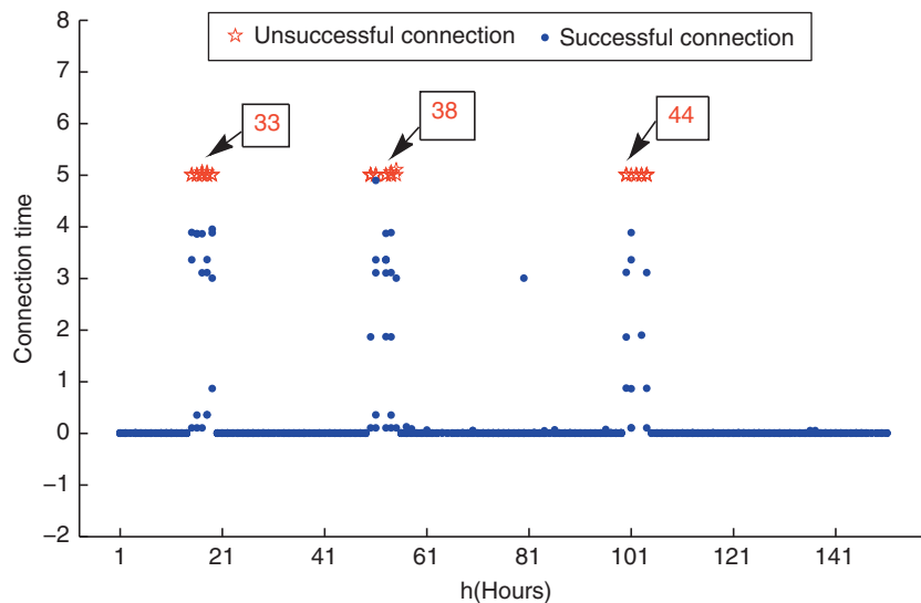
Figure 3.8 The unsuccessful and successful connections and their elapsed times between MTU and PLC_6 .
