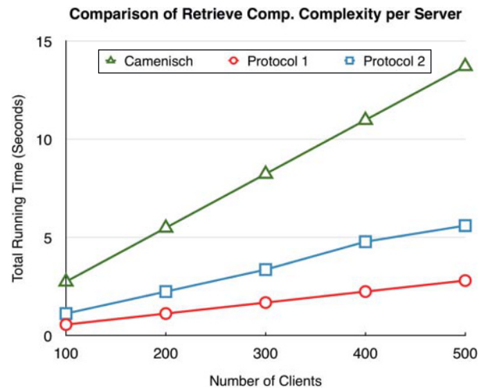
Figure 7.8 Comparison of average time spent by a server in retrieving.
