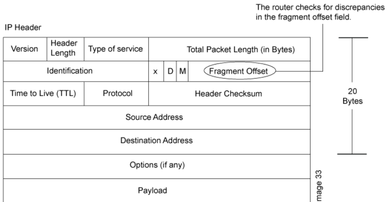
Figure 11: Teardrop Attacks
