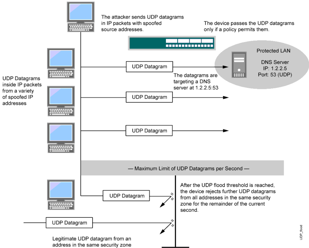
Figure 8: UDP Flooding
