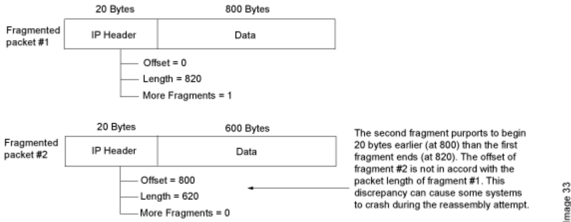
Figure 12: Fragment Discrepancy
