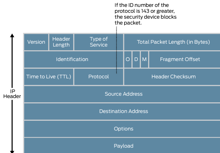
Figure 21: Unknown Protocols
