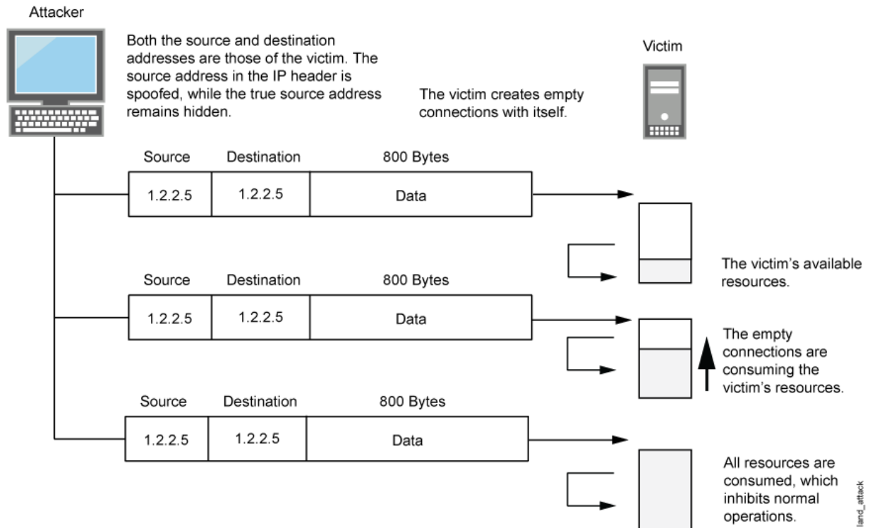
Figure 9: Land Attack
