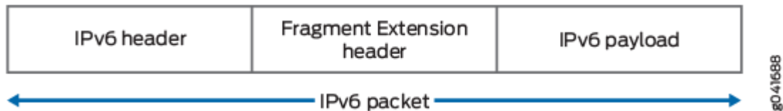
Figure 18: IPv6 Packet
