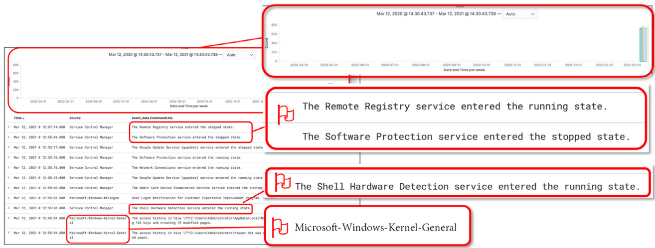
Kibana Discover Pane: Event Data for Host 213.239.209.202, highlighting evidence of Command-and-Control activity
