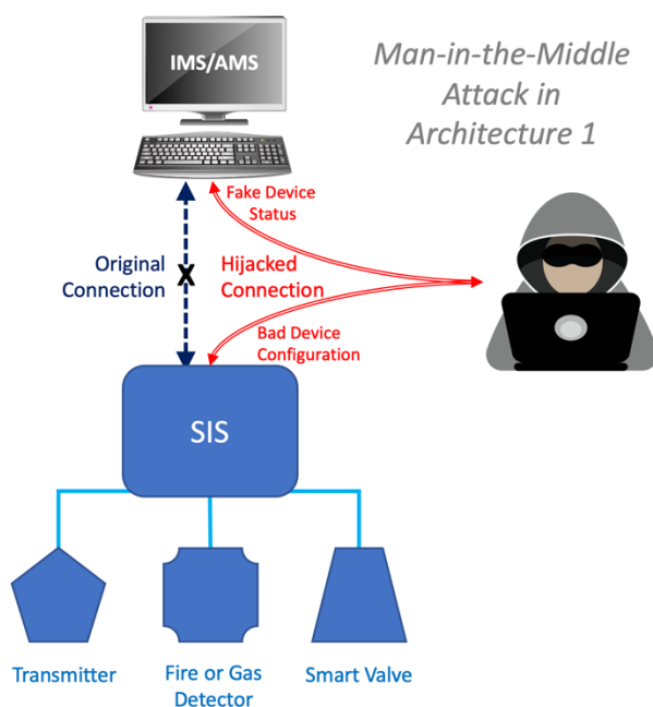
Figure 7. Under certain conditions, unencrypted communications can be hijacked by attackers and used to block or change operator-initiated device commands and send false device status to the IMS/AMS operator console. Using alternate techniques, a similar capability could be achieved through co-resident malware running directly on the IMS/AMS.
