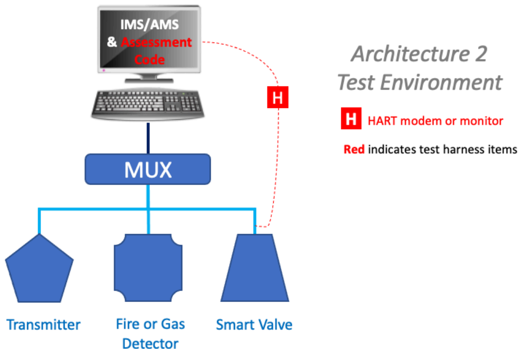
Figure 4. The Architecture 2 test environment consisted of multiple instruments, an IMS/AMS, a MUX, and test harness components. Testcases were launched from the IMS/AMS platform as co-resident processes with the IMS/AMS software.
