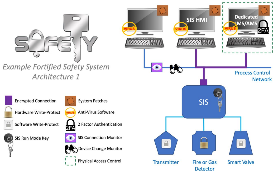
Figure 8. Manage risk by implementing a layered, defense-in-depth approach that fortifies safety systems and their operating environments against network-based, insider, and supply-chain attacks.
