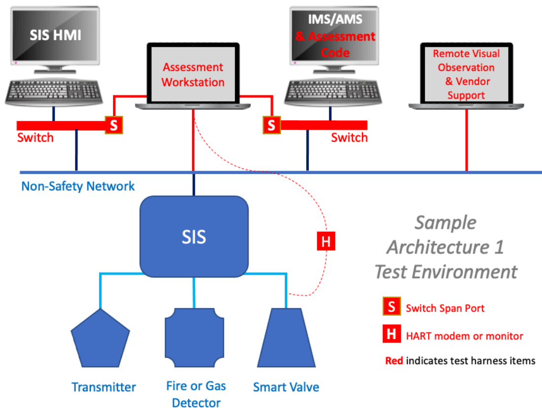
Figure 3. The Architecture 1 test environment consisted of multiple instruments, an IMS/AMS, an SIS, an SIS HMI, and test harness components (shown in red). Each environment differed slightly based on vendor product solutions.
