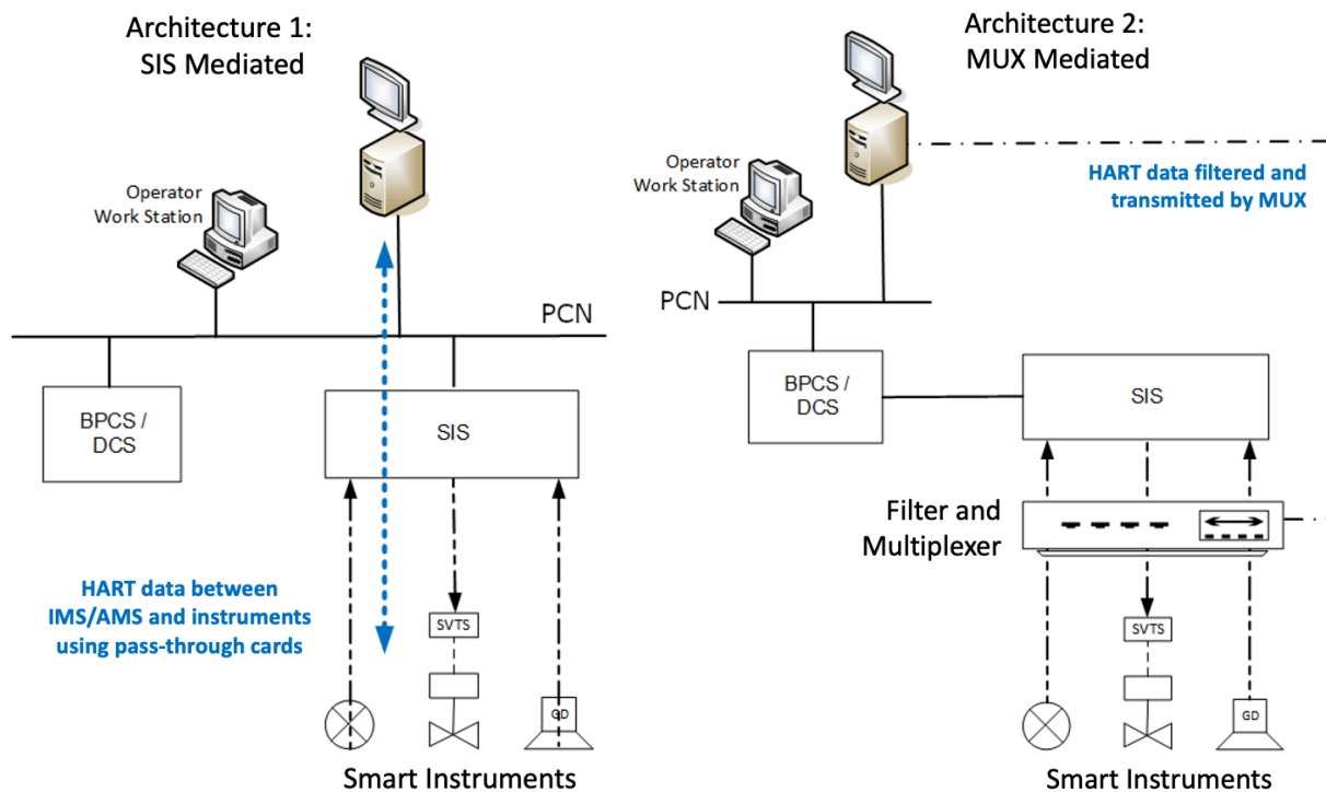
Figure 2. Architecture 1 (left) provides direct network connection to the SIS, which mediates communications between the IMS/AMS and devices. In contrast, the SIS in Architecture 2 (right) is accessed through an interface on the BPCS/DCS and the IMS/AMS communicates with devices through a serial connection with a MUX.
