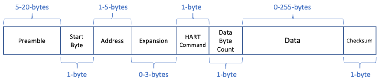
Figure 6. The request HART packet structure has a preamble field (for synchronization and carrier detect), a start delimiter (that designates the start of the communications packet), the device address, an expansion field, a numerical value designating a HART command, a size field for the data, a data field, and a 1-byte checksum for packet integrity.
