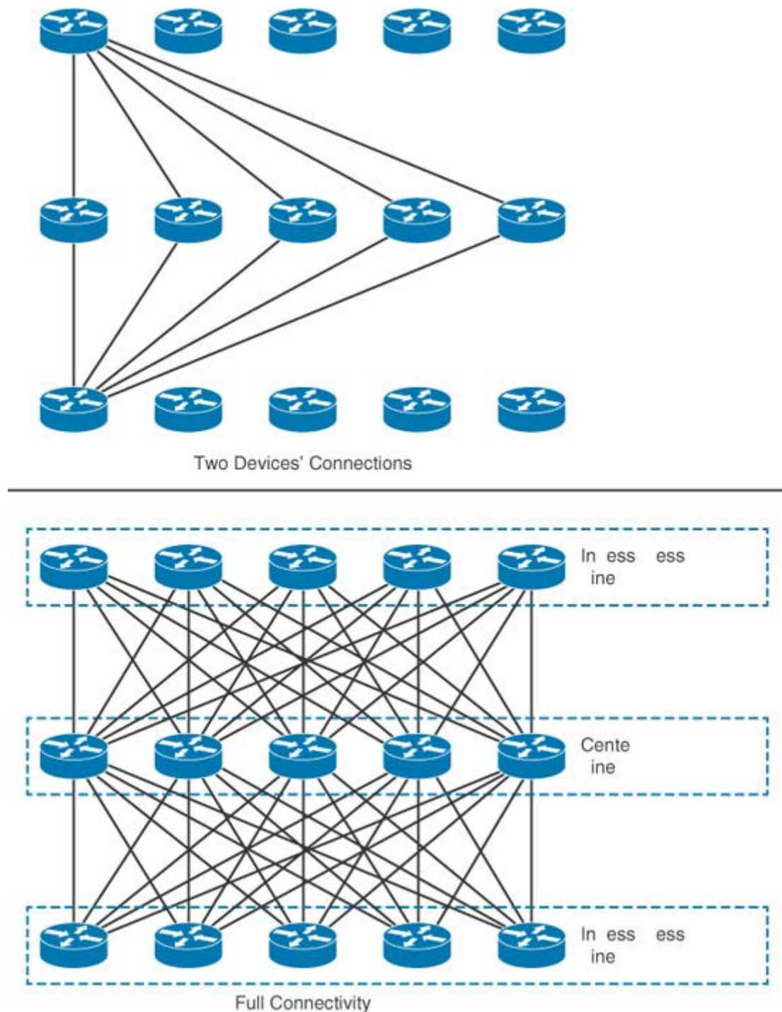
Figure 11-7 Clos Fabric
