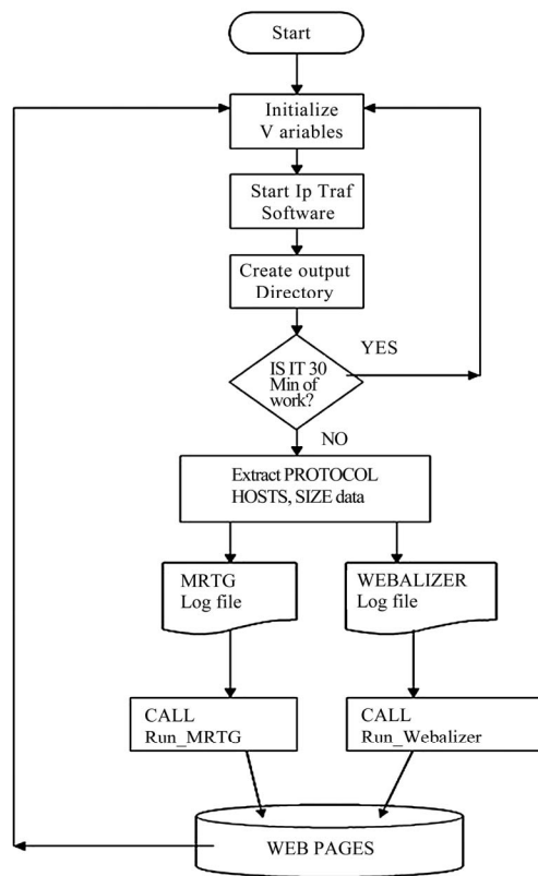
Figure 5. Wrapper script.
