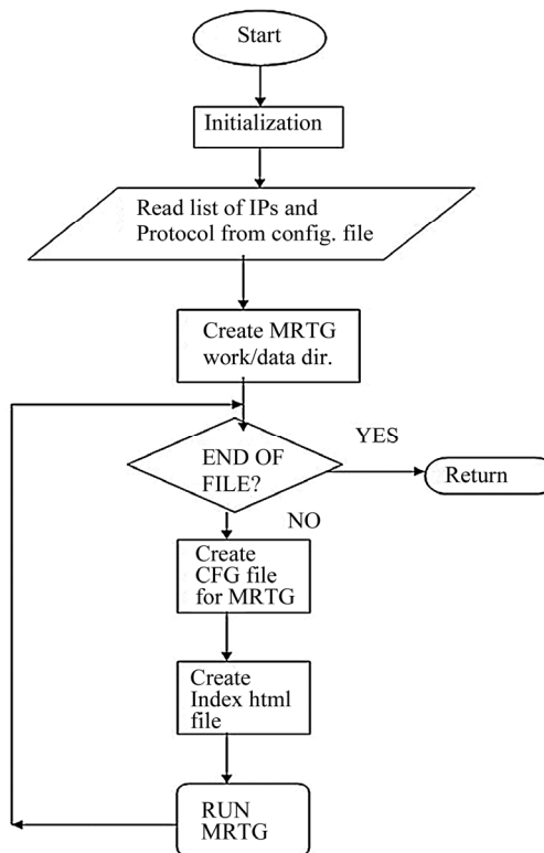
Figure 6. Run_mrtg script.
