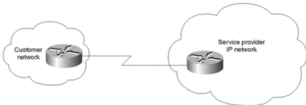
Figure 2-1. Dedicated Internet Access Configuration
