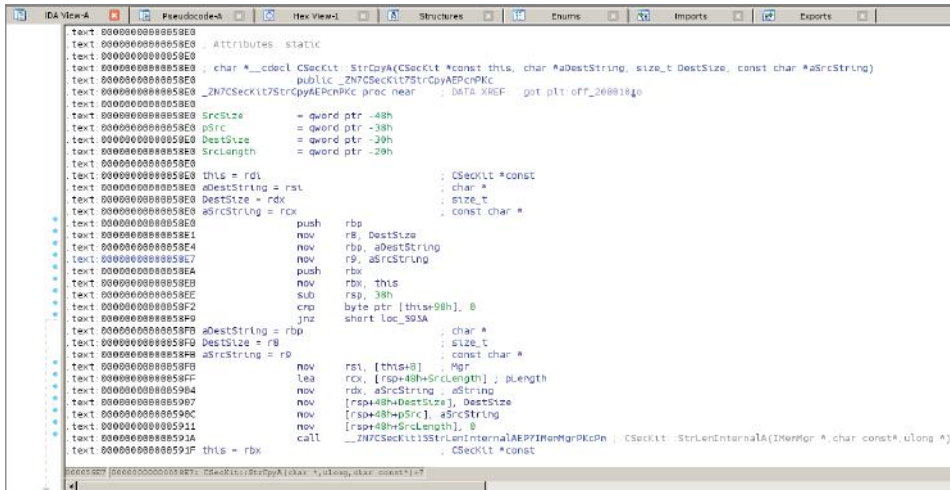
Figure 2-4: Disassembly of Comodo for Linux library libPE32.so showing full symbols
