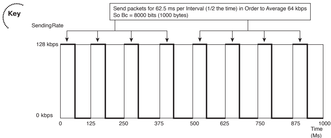
Figure 5-1 Mechanics of Traffic Shaping—128-kbps Access Rate, 64-kbps Shaped Rate
