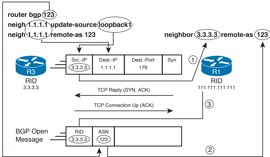
Figure 1-3 BGP Neighbor Parameter Checking
