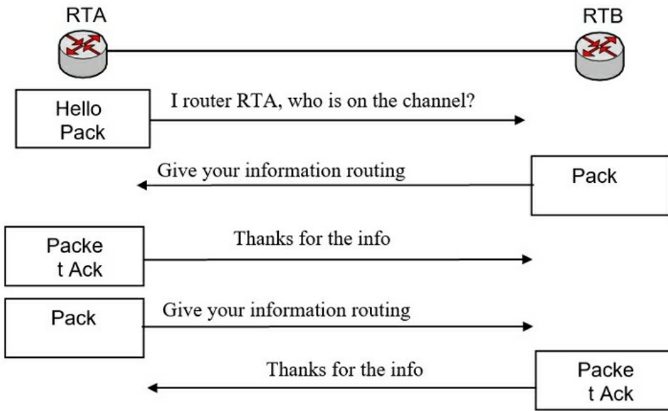
Exchange of information neighboring EIGRP routers
