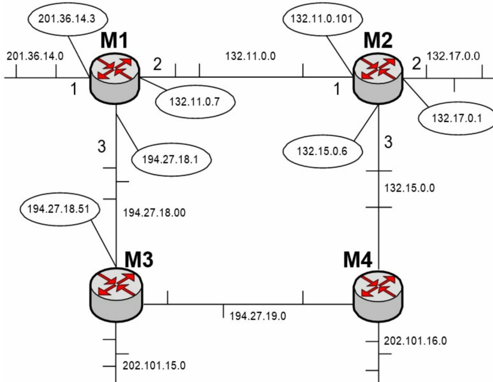
Network combined RIP-routers
