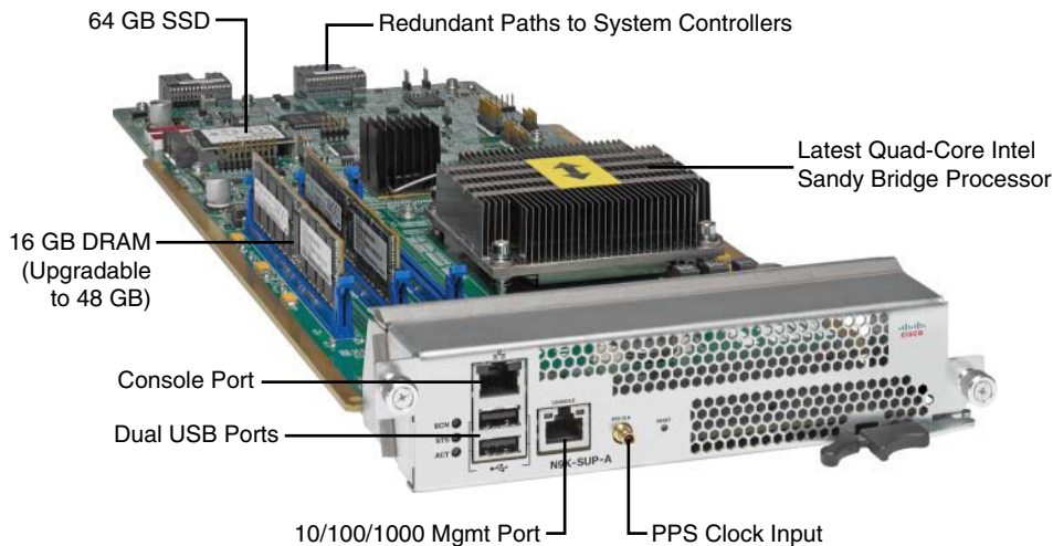
Figure 1-10 Nexus 9500 Supervisor Engine
