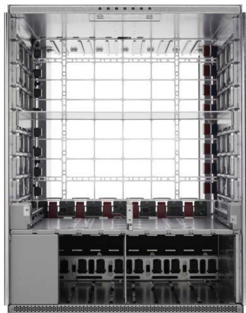
Figure 1-9 Nexus 9500 Chassis
