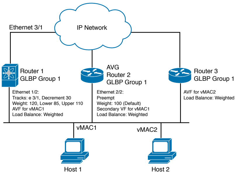
Figure 20-12 GLBP Topology
