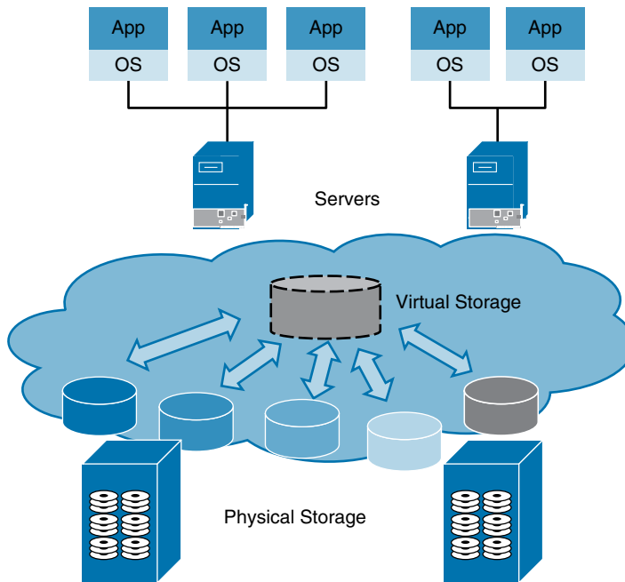
Figure 23-1 Storage Virtualization Mapping Heterogeneous Physical Storage to Virtual Storage
