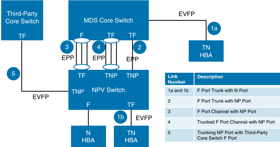
Figure 23-36 Trunking F Ports
