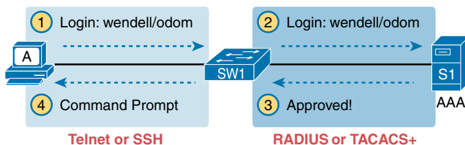
Figure 10-2 Basic Authentication Process with an External AAA Server
