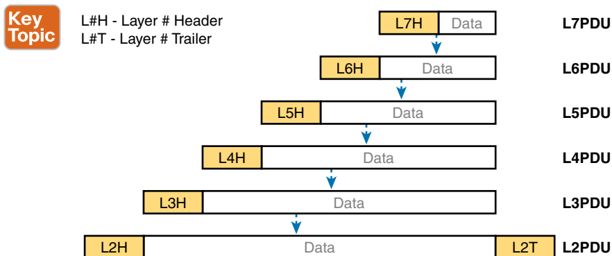
Figure 2-16 OSI Encapsulation and Protocol Data Units
