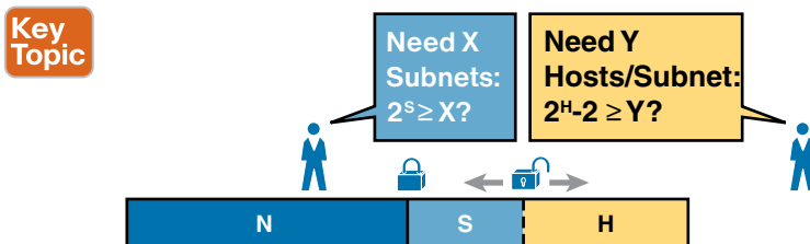
Figure 11-18 Borrowing Enough Subnet and Host Bits
