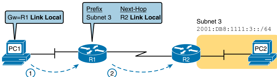
Figure 15-12 IPv6 Using Link Local Addresses as the Next-Hop Address
