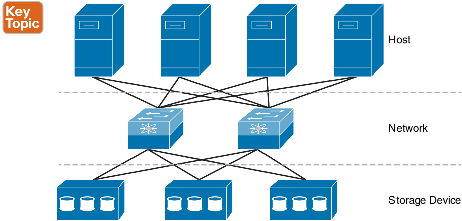
Figure 23-3 Possible Alternatives Where the Storage Virtualization May Occur
