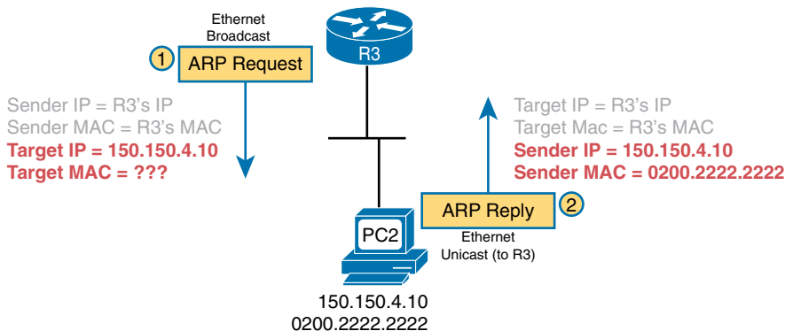
Figure 4-14 Sample ARP Process
