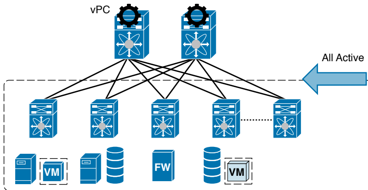
Figure 1-4 Virtual Port Channel (vPC)
