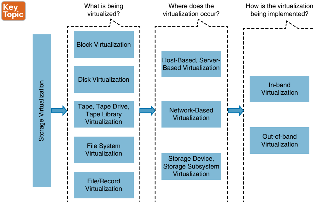
Figure 23-2 SNIA Storage Virtualization Taxonomy Separates Objects of Virtualization from Location and Means of Execution
