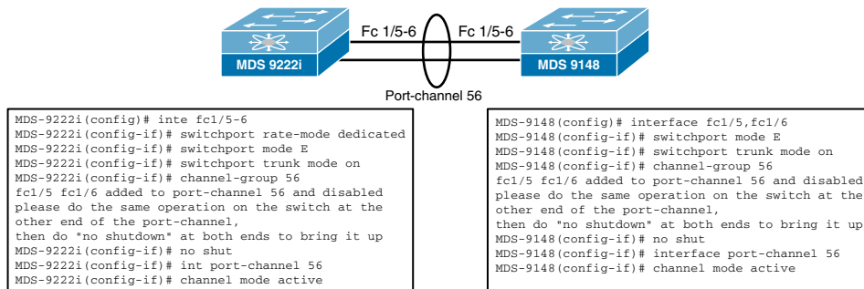
Figure 23-37 Setting Up ISL Port on Sample SAN Topology
