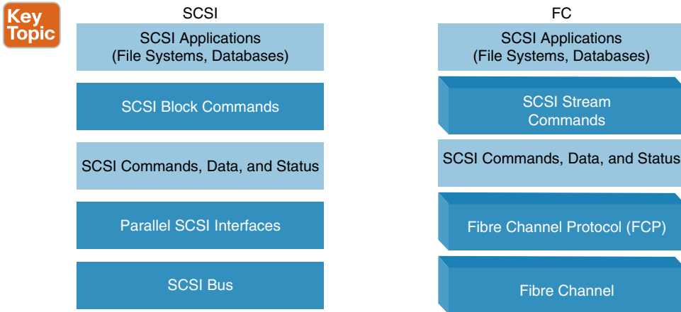
Figure 22-31 FCP Protocol Stack
