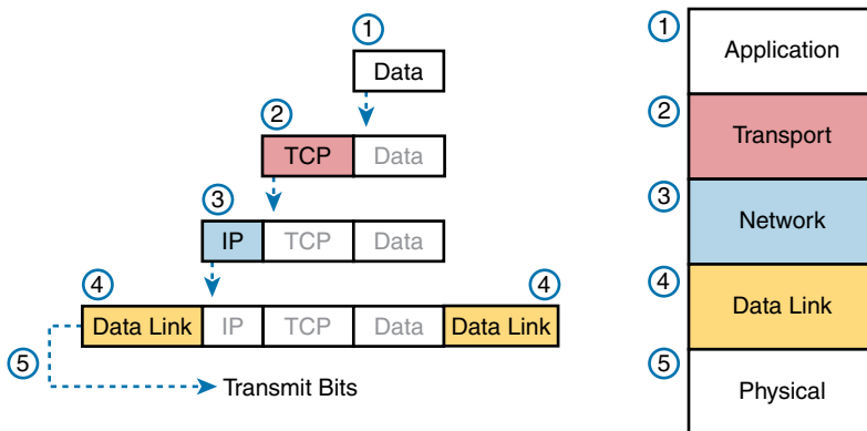
Figure 2-13 Five Steps of Data Encapsulation: TCP/IP
