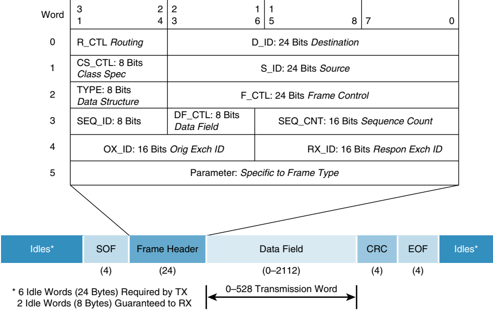
Figure 22-24 Fibre Channel Frame Format
