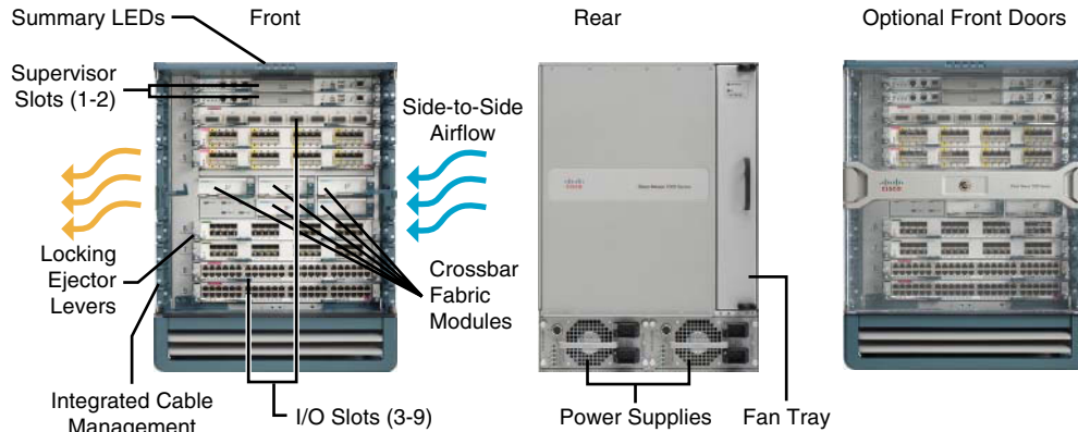
Figure 1-20 Cisco Nexus 7009 Switch
