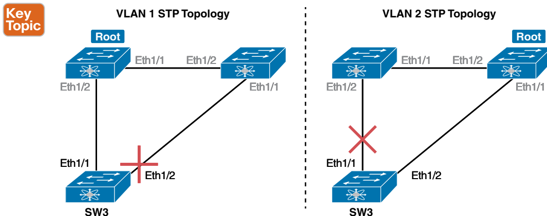
Figure 9-2 Load Balancing with PVST+
