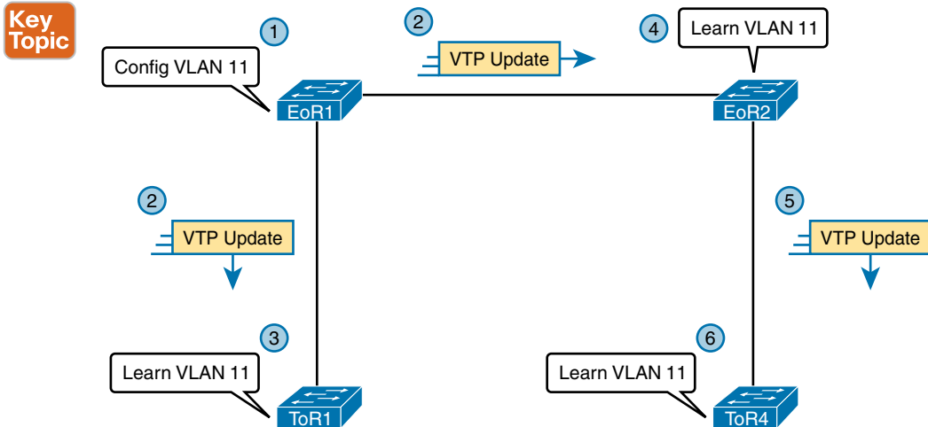
Figure 6-13 A VTP Example of Configuring and Synchronizing for New VLAN 11
