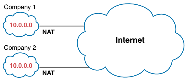
Figure 11-15 Reusing the Same Private Network 10.0.0.0, with NAT
