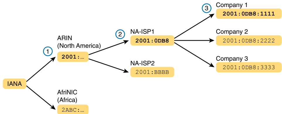
Figure 15-5 Prefix Assignment with IANA, RIRs, and ISPs
