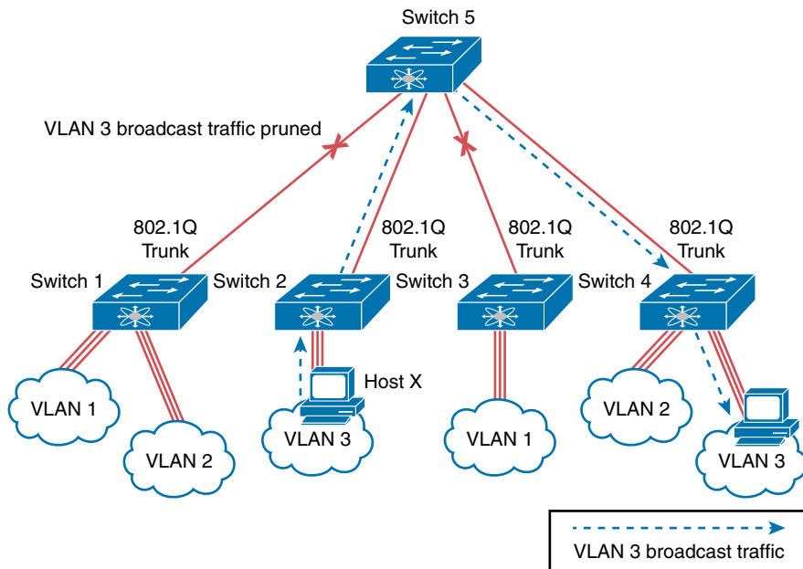
Figure 7-5 VTP Pruning
