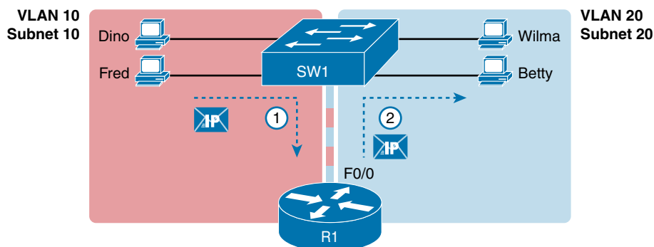
Figure 6-9 Routing Between Two VLANs Using a Trunk on the Router
