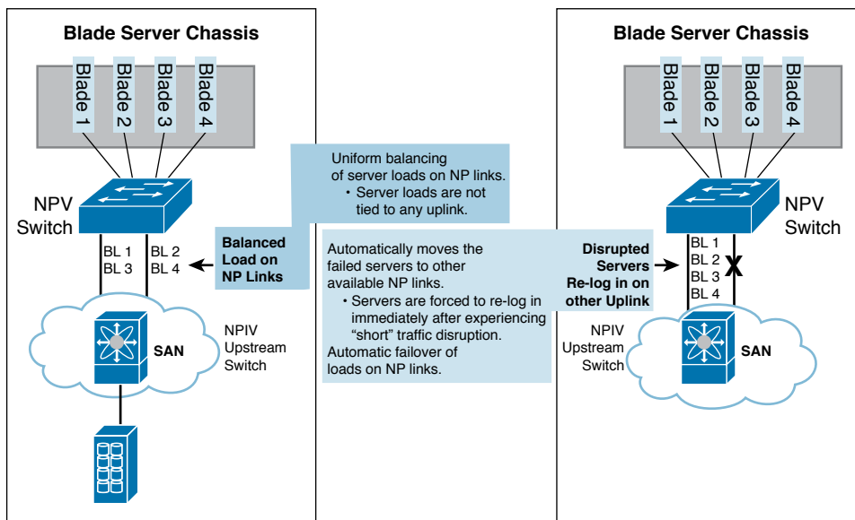
Figure 23-18 NPV Auto Load Balancing
