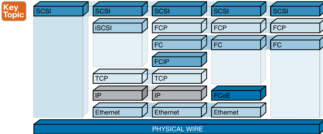
Figure 22-8 Networking Stack Comparison for All Block I/O Protocols
