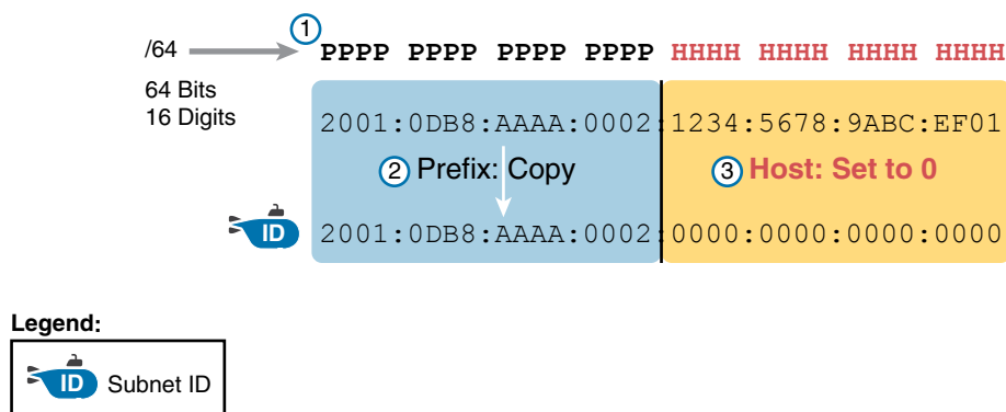
Figure 15-3 Creating the IPv6 Prefix from an Address/Length
