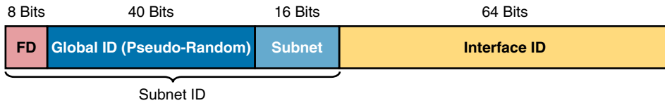
Figure 15-11 IPv6 Unique Local Unicast Address Format
