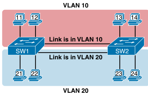
Figure 6-3 Multiswitch VLAN Without VLAN Trunking
