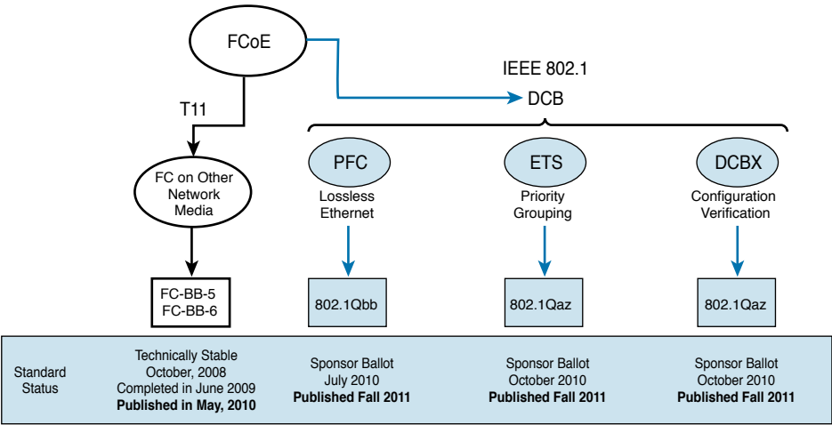
Figure 23-47 Standards for FCoE
