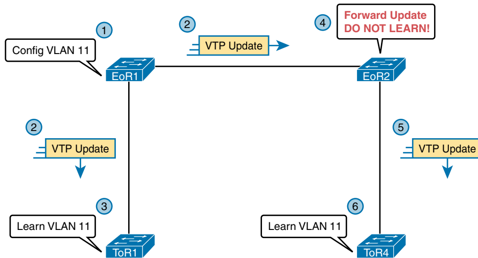
Figure 6-14 The Need for VTP Transparent Mode
