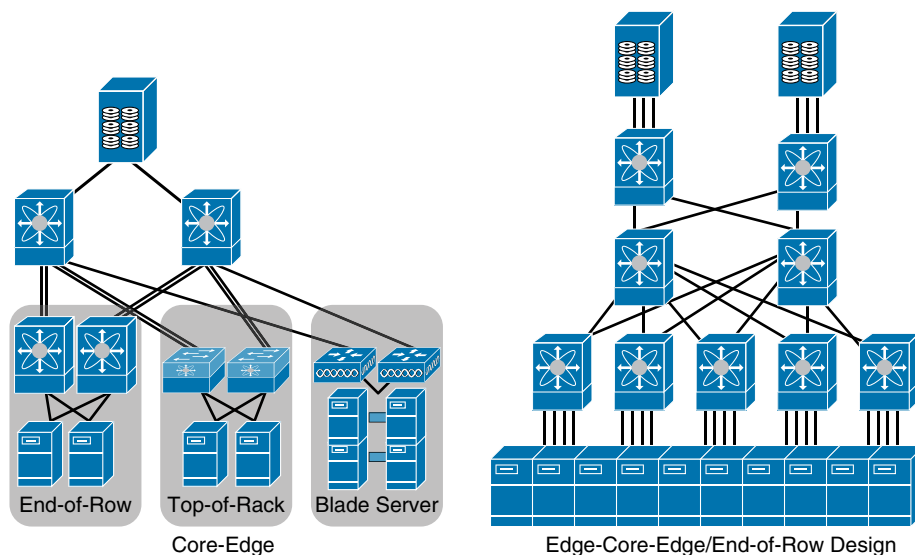
Figure 22-20 Sample FC SAN Topologies
