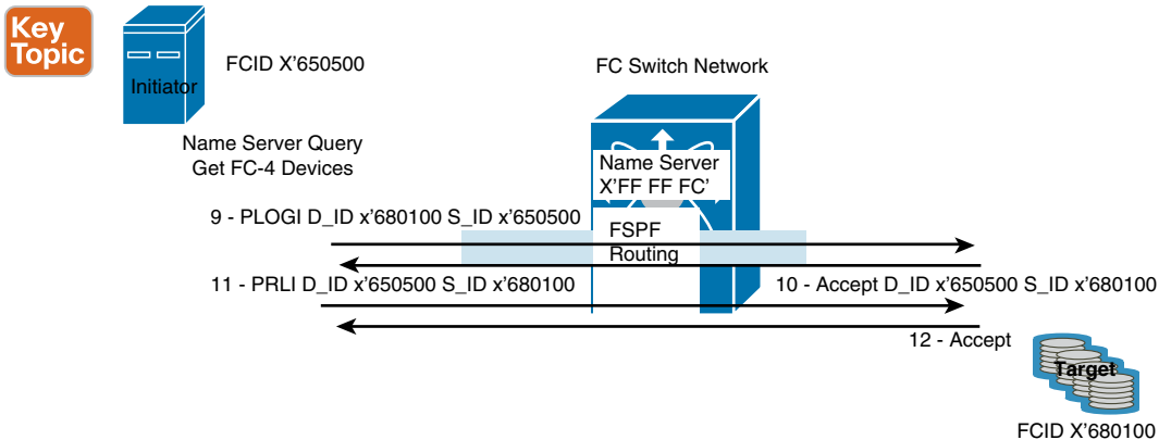
Figure 22-30 Fibre Channel Port/Process Login to Target
