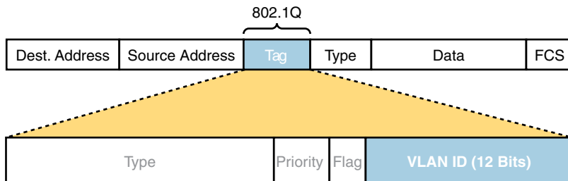
Figure 6-6 802.1Q Trunking
