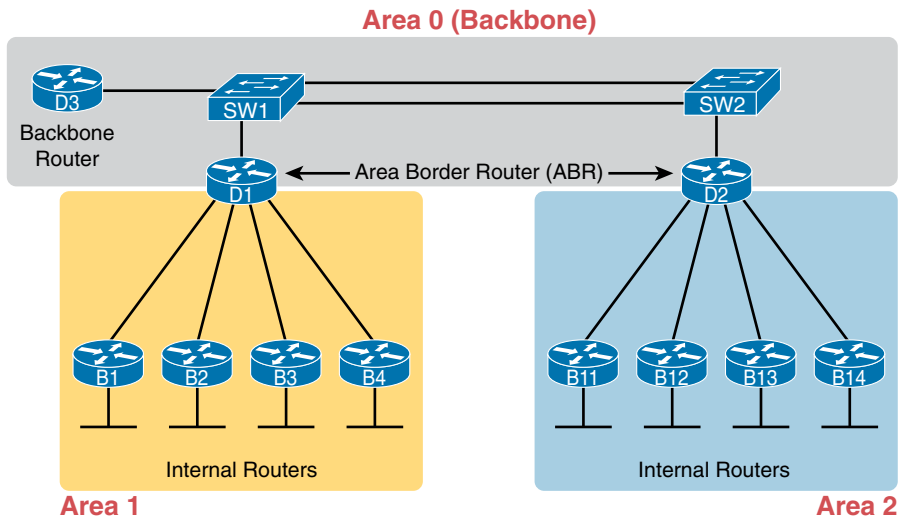
Figure 18-16 Three-Area OSPF
