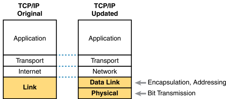
Figure 2-12 Link Versus Data Link and Physical Layers
