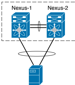
Figure 20-13 vPC Topology
