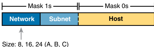
Figure 13-6 Class Concepts Applied to Create Three Parts
