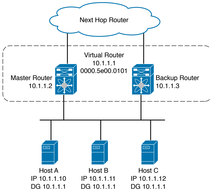
Figure 20-11 VRRP Topology
