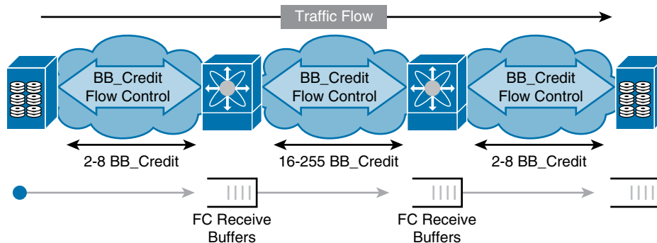
Figure 22-26 Fibre Channel Frame Buffering
