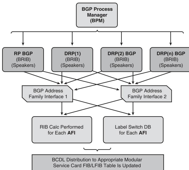
Figure 8-2 Distributed BGP
