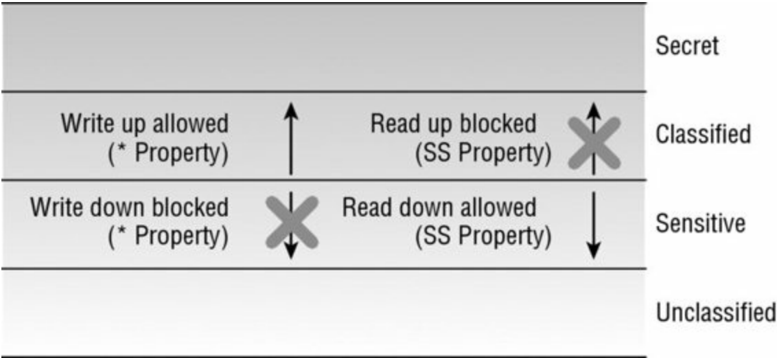
Figure 8.3 The Bell-LaPadula model
