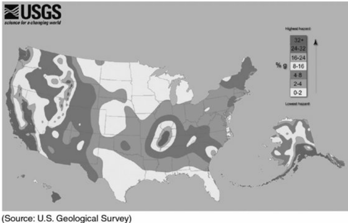
Figure 3.1 Earthquake hazard map of the United States
