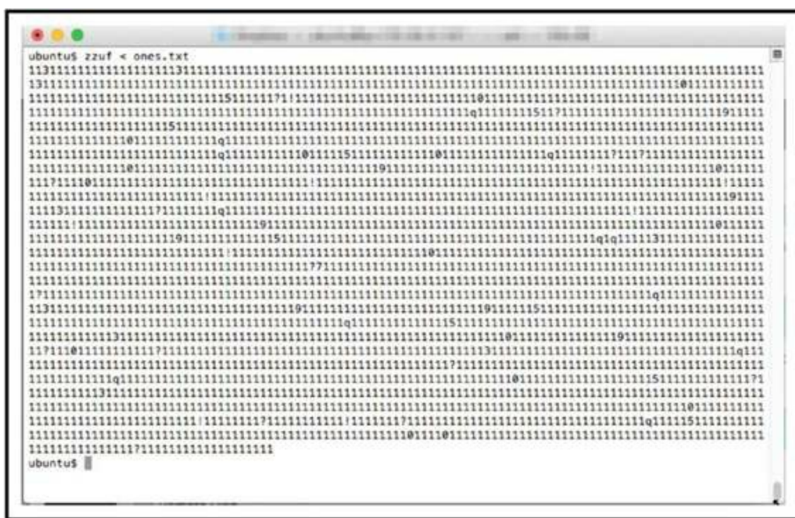
Figure 15.9 :The input file from Figure 15.8 after being run through the zzuf mutation fuzzing tool
