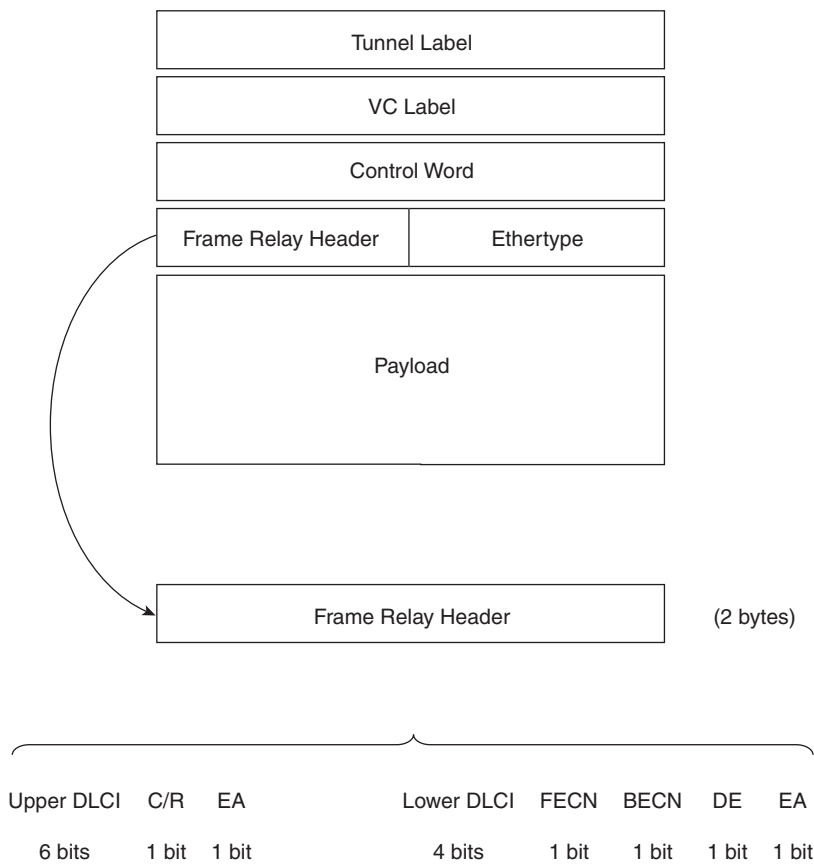
Figure 10-12 Port-to-Port FRoMPLS Frame Format for Cisco Encapsulation
