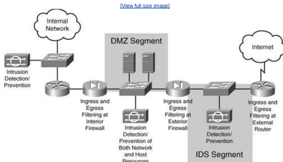
Figure 9-5. Dual-Firewall System
