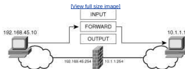
Figure 7-2. NetFilter FORWARD Chain Processing
