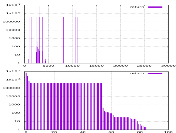
Figure 2. Distribution of return table for sqlite3, unsorted and sorted. The x-axis represents the distinct return instructions. Note the y-axis scale, and the different range on the x-axis: the bottom graph is a zoom on executed return instructions. All others are never executed.
