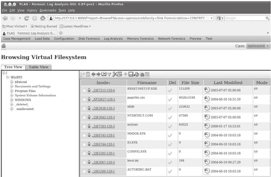
FIGURE 9.3 PyFLAG—file system browsing.
