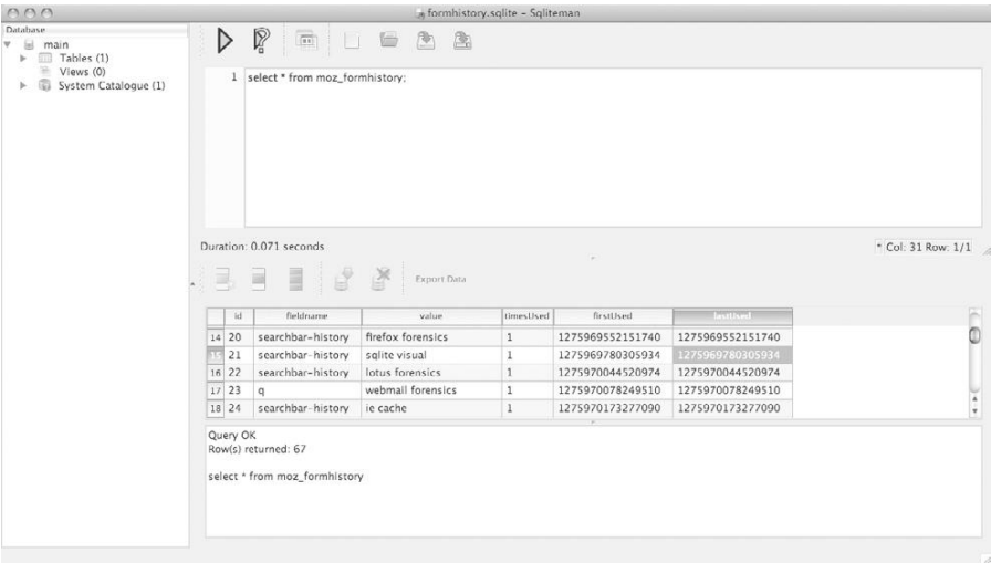
FIGURE 7.2 SQLite query for moz_formhistory.
