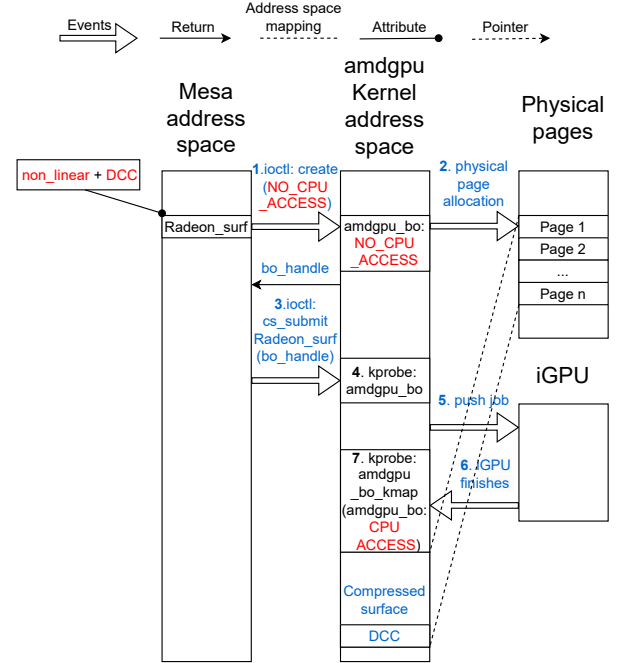
Figure 10. Mesa and amdgpu trace of texture creation. For the texture created in our minimal OpenGL program, amdgpu allocates a buffer object amdgpu_bo with a NO_CPU_ACCESS flag (1, 2). Mesa submits a non-blocking command to the iGPU for filling it (3–5). After the iGPU writes to the amdgpu_bo , we remove the NO_CPU_ACCESS attribute, then force a kernel address space mapping by invoking amdgpu_bo_kmap() to force a kernel mapping (6, 7) that we can dump.
