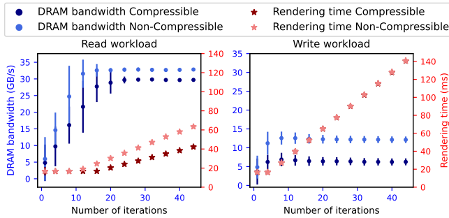
Figure 3. DRAM bandwidth (GB/s) and rendering time (ms) vs. iterations on our Intel i7-8700 when running the read workload (left) and write workload (right) on compressible and non-compressible patterns. The read workload generates enough traffic to saturate the iGPU memory subsystem. As a result, traffic reduction due to compression leads to a proportional reduction in the rendering time of compressible patterns. The write workload does not saturate the iGPU memory subsystem. The rendering time delay is due to running out of iGPU computation resources. Therefore, DRAM bandwidth differences are not reflected in the rendering time.
