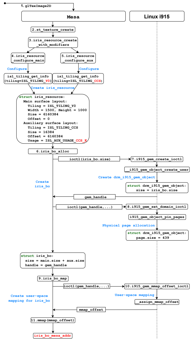
Figure 18. Complete Mesa and i915 trace of tile-Y formatted texture creation in our minimal OpenGL program from Section 4.1. Upon texture creation ( glTexImage2D ), Mesa configures a data structure iris_resource that records the necessary information of a tile-Y formatted main surface and its CCS auxiliary surface. Mesa issues ioctl calls to i915 to create and allocate a buffer object drm_i915_gem_object that represents the texture in the kernel space. Then, Mesa requests a userspace mapping of the drm_i915_gem_object and maps it at address iris_bo_mesa_addr . Once the iGPU completes writing to drm_i915_gem_object , iris_bo_mesa_addr contains the compressed tile-Y formatted main surface, and iris_bo_mesa_addr plus an offset contains the auxiliary CCS.
