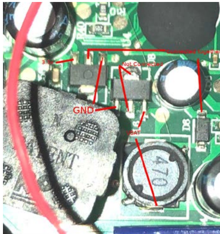
Figure 3.2 – Probing the power section chips
