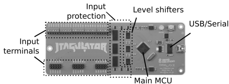
Figure 10.3 – The JTAGulator
