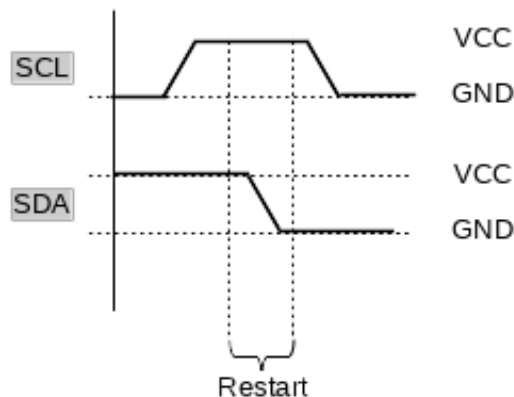
Figure 6.6 – I2C restart condition
