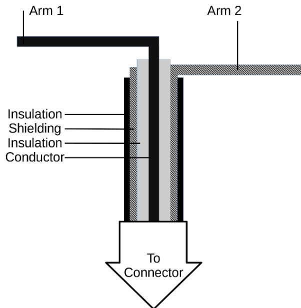
Figure 9.1 – Dipole antenna connection
