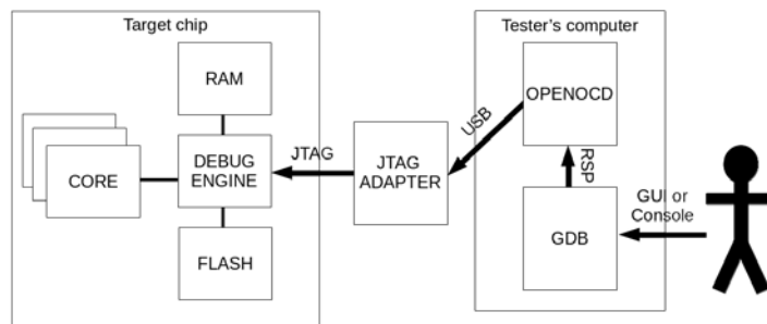
Figure 12.1 – Debug chain
