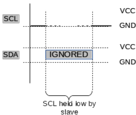
Figure 6.7 – I2C pause
