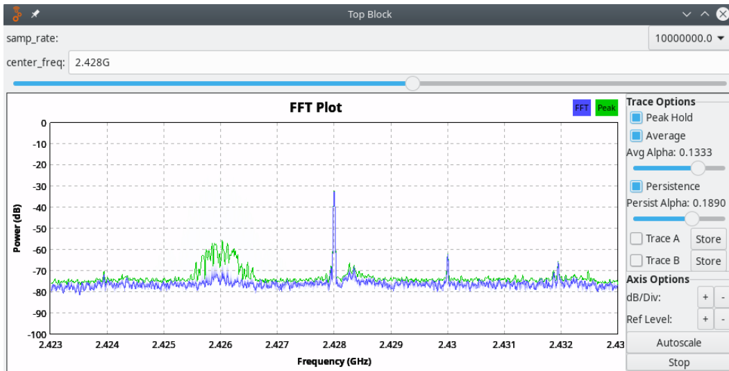
Figure 9.6 – A typical FFT plot (here, centered on Wi-Fi frequencies)
