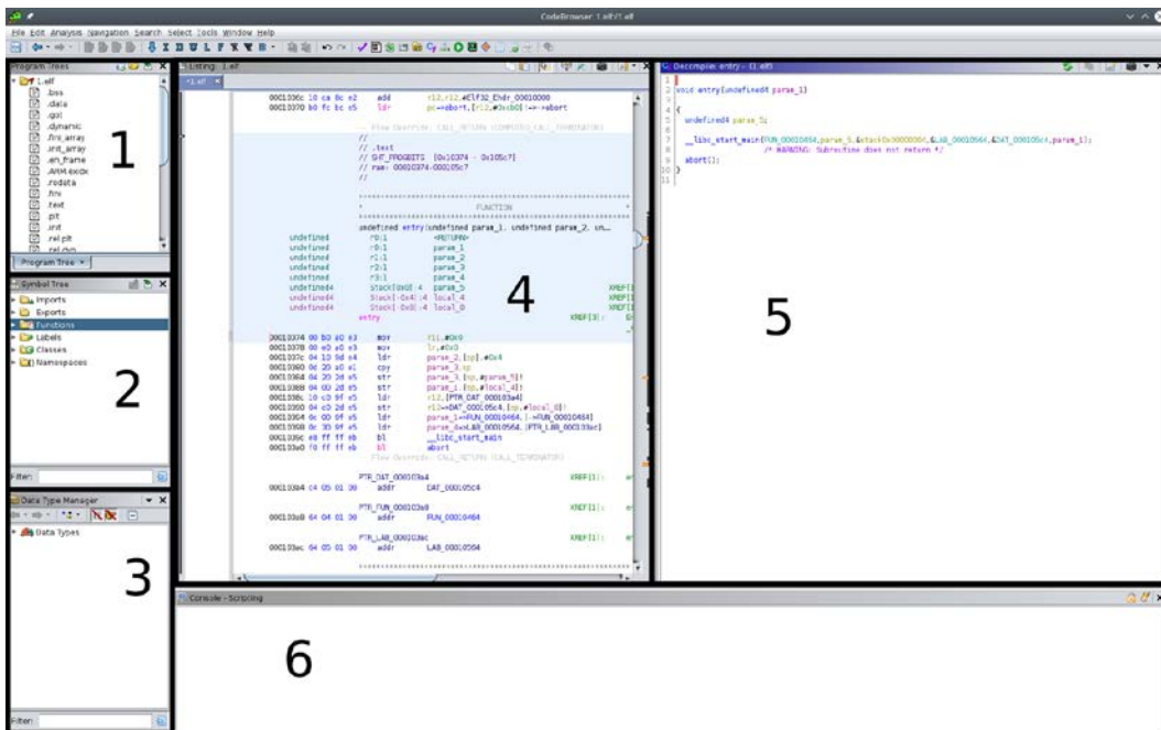
Figure 11.4 – Ghidra layout
