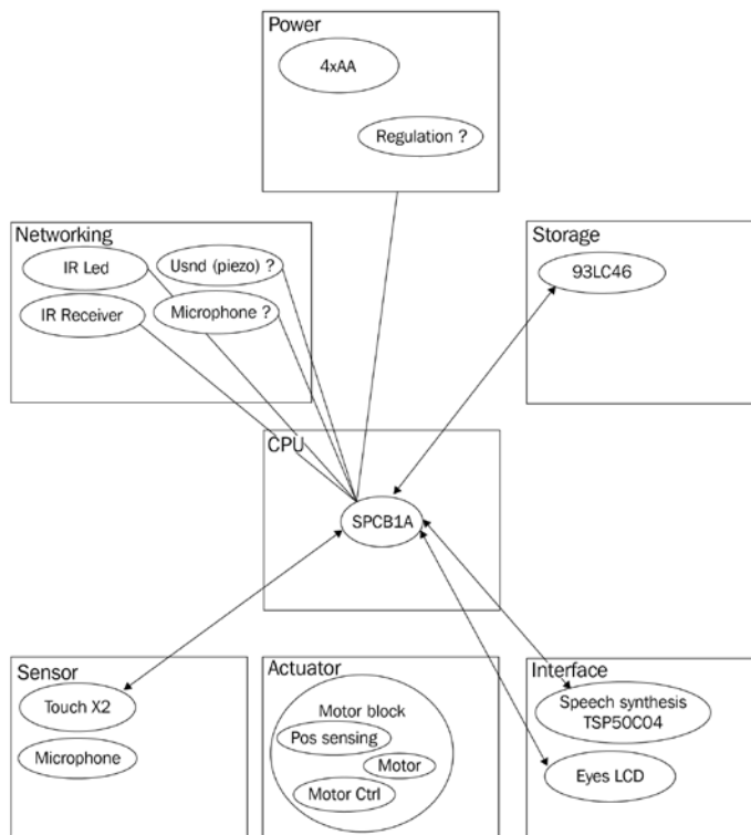
Figure 3.1 – Components in blocks
