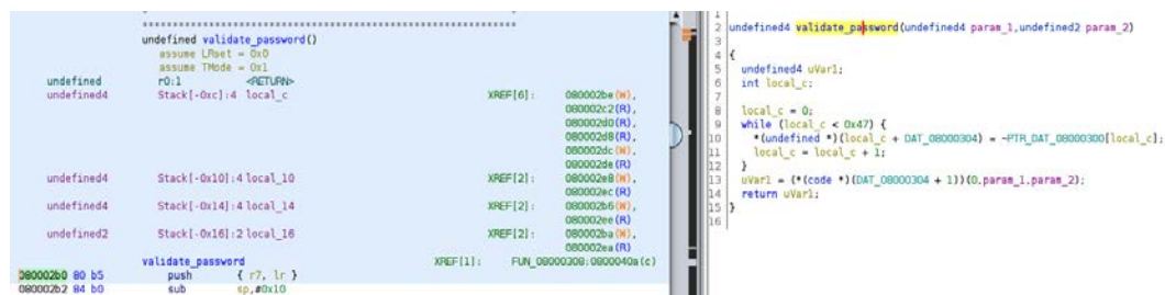
Figure 12.3 – Finding a function address in Ghidra
