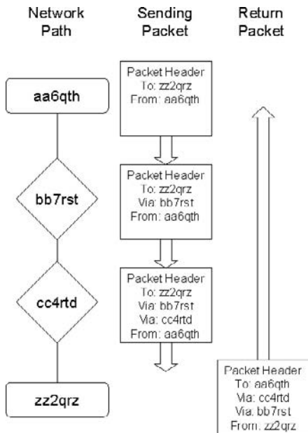
FIGURE 11.2 AX.25 address routing.
