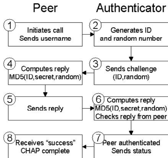
FIGURE 9.1 CHAP processing.
