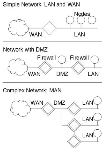
FIGURE 6.1 The four network regions: LAN, MAN, DMZ, and WAN.
