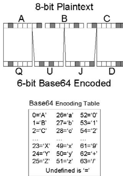
FIGURE 4.1 Base64 encoding.
