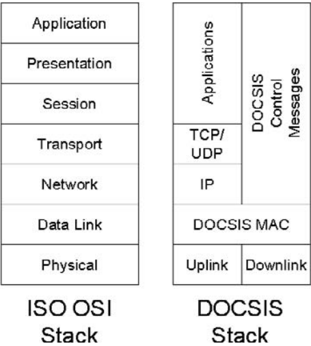
FIGURE 3.2 Aligning the DOCSIS and OSI network stacks.
