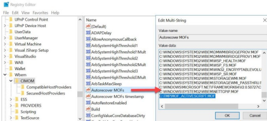
Figure 22: Autorecover MOFs Registry Key
