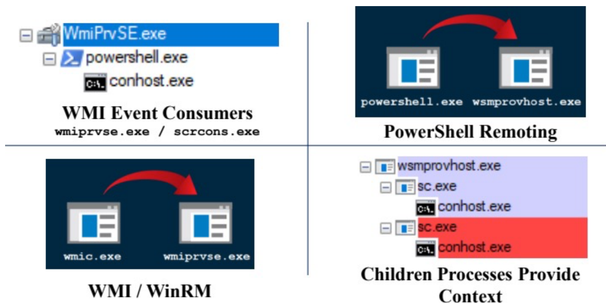
Figure 23: WMI and PowerShell Processes
