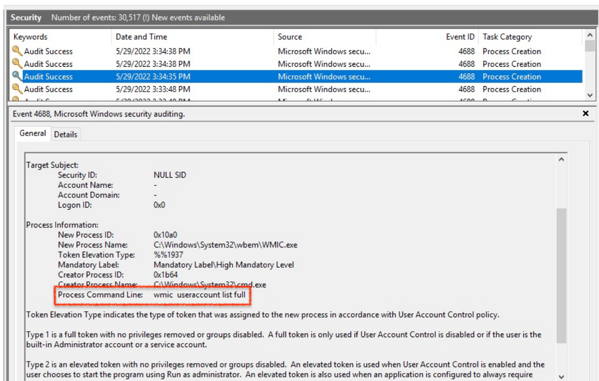
Figure 8: Event ID 4688 (Process Creation)
