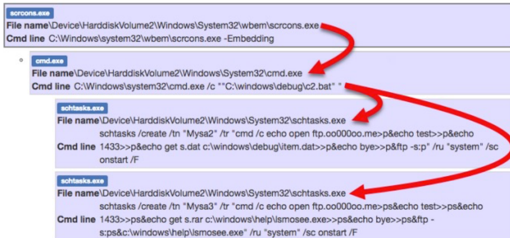
Figure 25: scrcons.exe Process Tree
