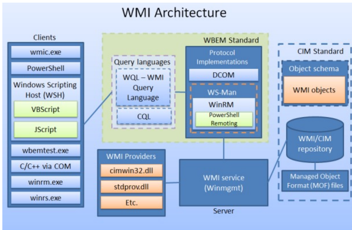
Figure 1: WMI Architecture
