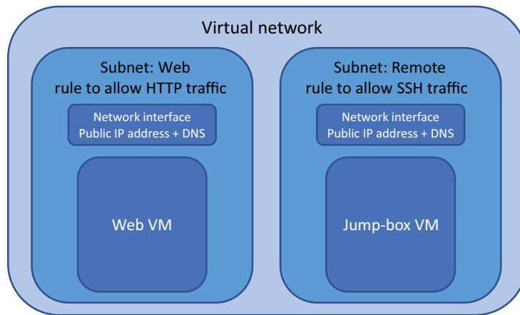
Figure 5.1 Software-defined network connections in Azure
