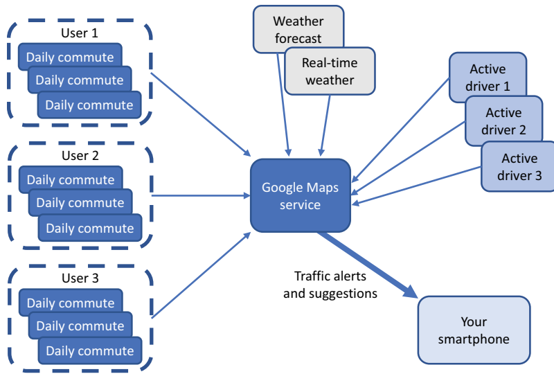
Figure 17.4 Each day, the Google Maps service receives multiple data points from users that record details of their commute. This data can be prepared and processed, along with the weather forecast and real-time weather during those commutes. ML algorithms can be applied to these large datasets and a data model produced. As a smaller sample of active drivers feed their current travel conditions or weather data into the Google Maps service, the data model can be applied to predict the commute and generate a traffic alert to their smartphones that suggests an alternative route home.
