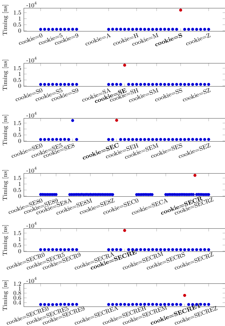
Figure 9.14.: Bitwise leakage of the secret (S,E,C,R,E,T) from ZRAM. Times for guesses (0-9, A-Z) for each of the bytes are shown. The highest value in each plot (shown in red) indicates the correct secret value for the byte. Standard error margins are below 1 % of the values and, thus, not visible in the plot.
