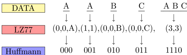
Figure 2.6.: Example for sequence compression using LZ77 and Huffmann encoding.
