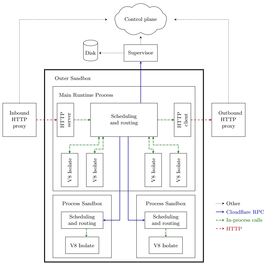
Figure 6.5.: DyPrIs overview.
