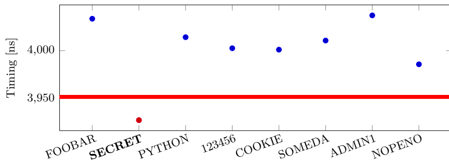
Figure 9.2.: Decompression time with Decomp+Time for different guesses of the secret value. A threshold (line) separating the correct from wrong secrets.
