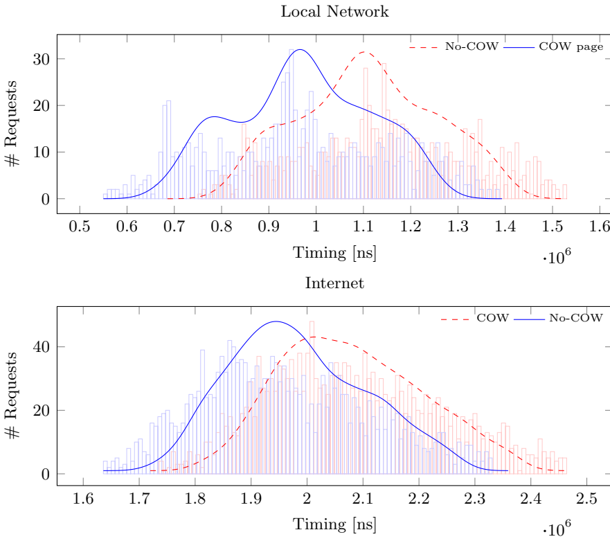
Figure 8.7.: Histogram of the network requests in a local area network and in the internet setup using 16 pages to amplify the results in Memcached.
