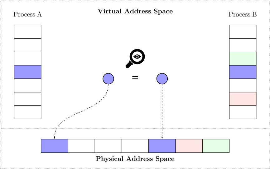
(a) Step 1: Find identical pages
