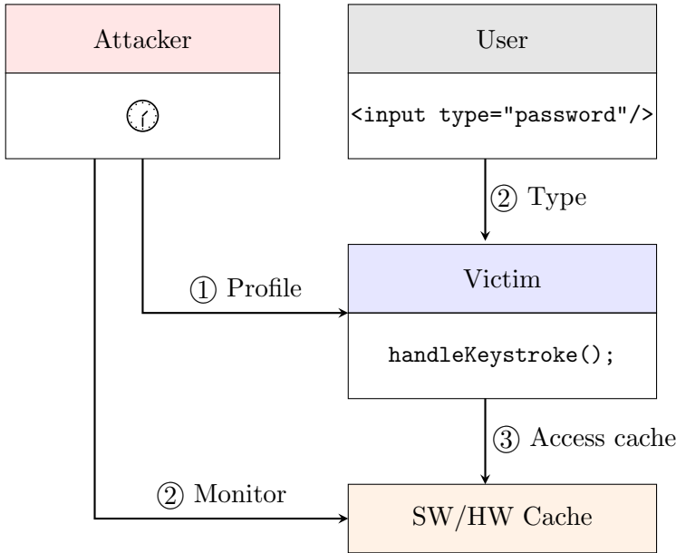
Figure 10.1.: Overview of the LBTA
