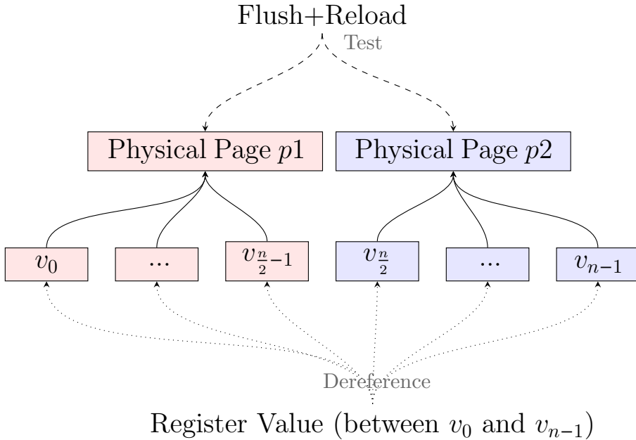
Figure 5.3.: Leaking the value of an x86 general-purpose register using Derefence Trap and Flush+Reload on two different physical addresses. v_0 to v_{n-1} represent the memory mappings on one of the shared memory regions.
