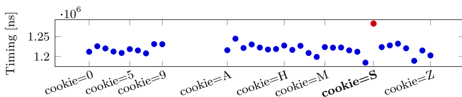
Figure 9.8.: Distribution of response times for the bitwise leakage in the remote PostgreSQL attack, with the correct guess (S) and incorrect guesses (0-9, A-R, T-Z). This is similar for subsequent bytes leaked (cf. Section E). Standard error margins are below 1% for all guesses and, thus, not visible in the plot.
