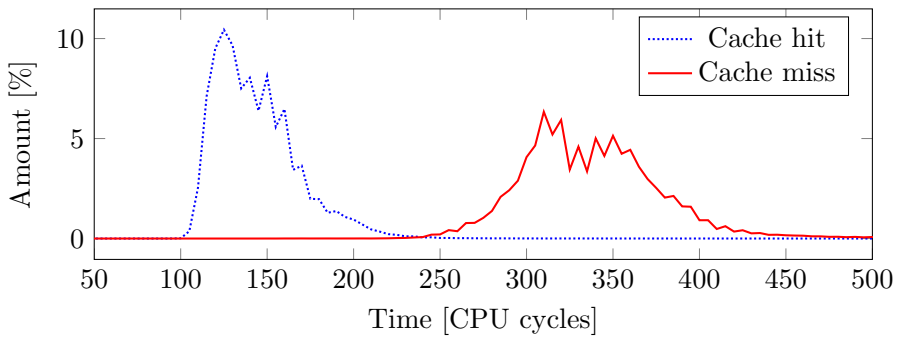
Figure 7.4.: Flush+Reload within a Specfuscator-compiled program works successfully as intended.
