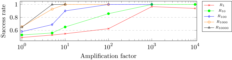
(b) Success of different amplification factors for different number of requests.
