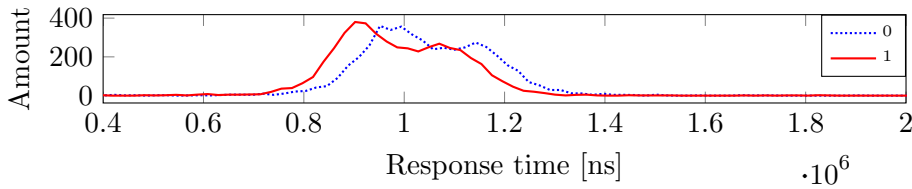
Figure 9.6.: Distribution of HTTP response times for zlib-decompressed pages stored in Memcached on memory compression encoding a ‘1’ and a ‘0’-bit.
