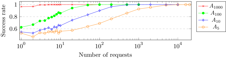
(a) Success over the number of requests per number of amplification factor.
