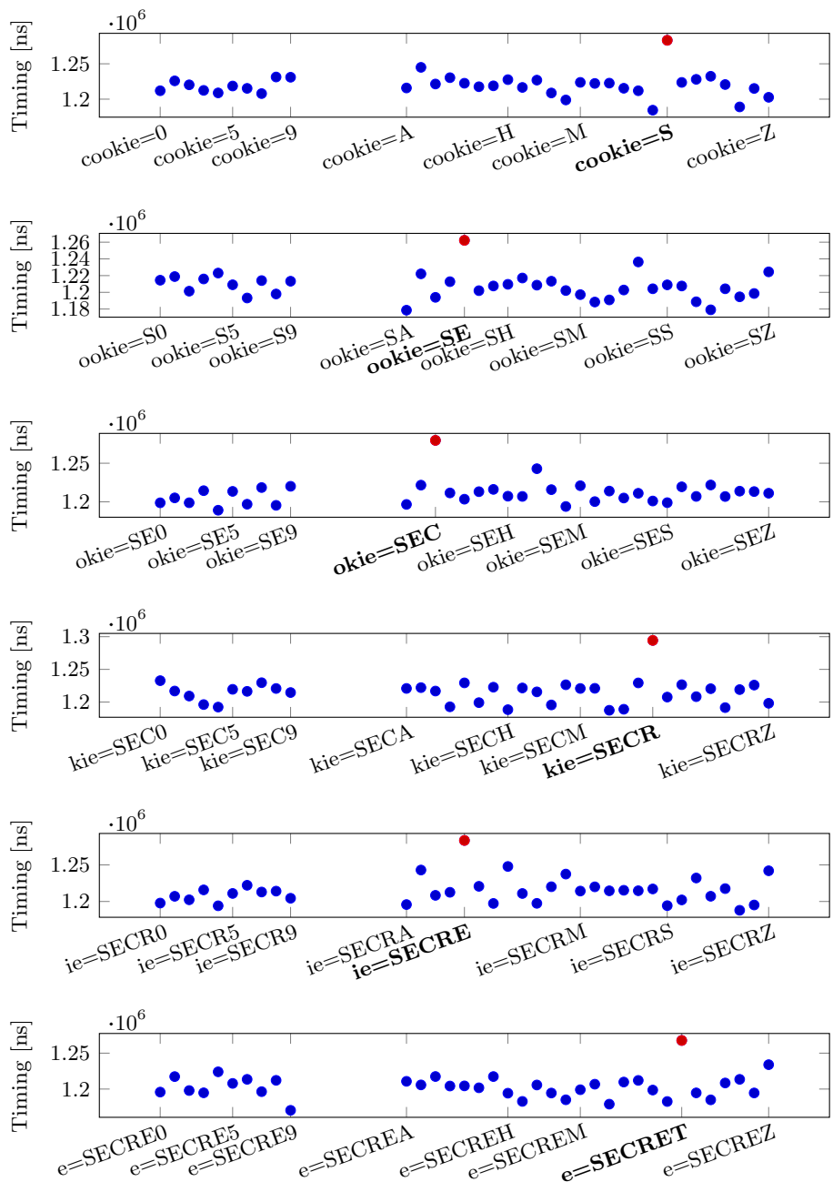
Figure 9.13.: Bitwise leakage of the secret (S,E,C,R,E,T) from PostgreSQL. The known prefix ( cookie= ) is shifted left by 1 character in each step, allowing the same memory layout to be reused. In each plot, the highest timing (shown in red) indicates the correct guess. Standard error margins are below 1 % of the values and, thus, not visible in the plot.
