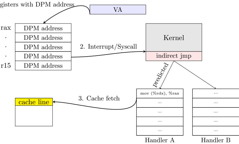
Figure 5.1.: The kernel speculatively dereferences the direct-physical map address. Flush+Reload detects cache hits on the corresponding user-space address.
