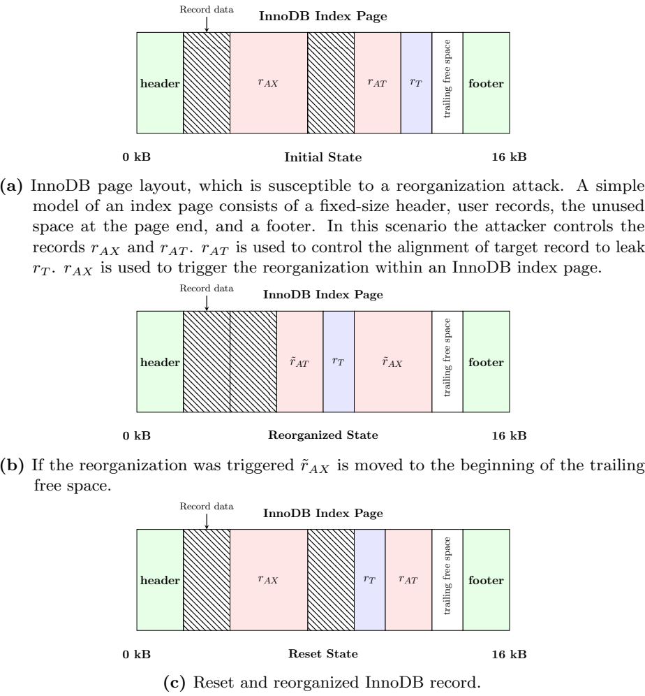
Figure 8.12.: InnoDB reorganization steps.
